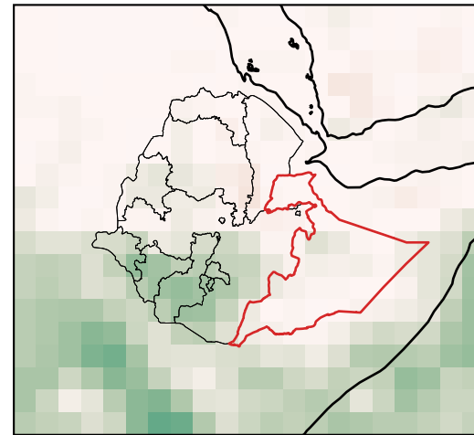
2007 MAM rainfall vs. 20% trigger threshold
