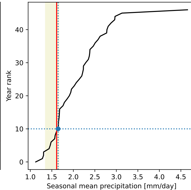
CDF of Somali region (Ethiopia) precipitation
