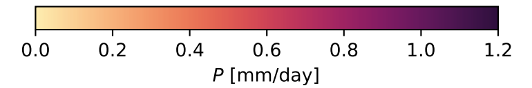
CDF of Somali region (Ethiopia) precipitation
