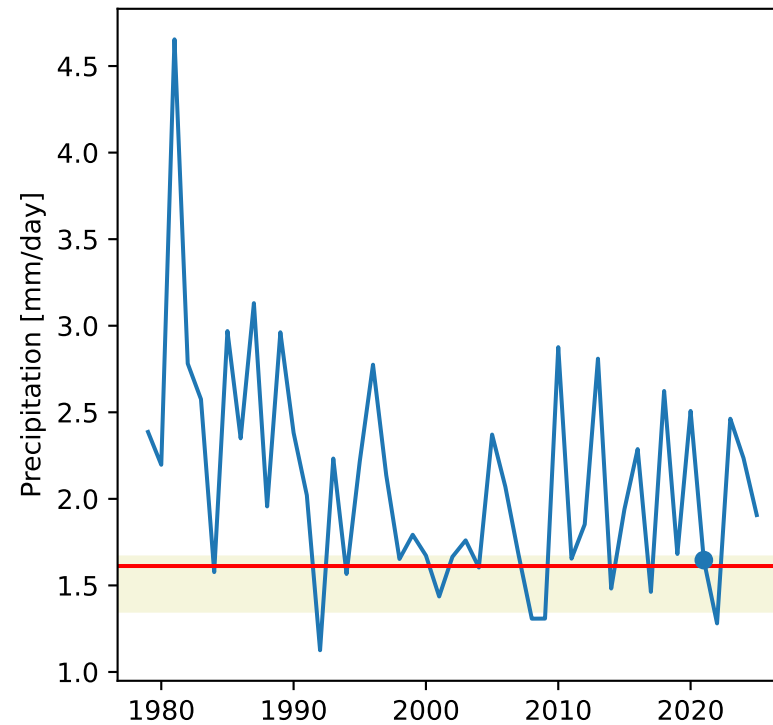
Somali region (Ethiopia) precipitation
