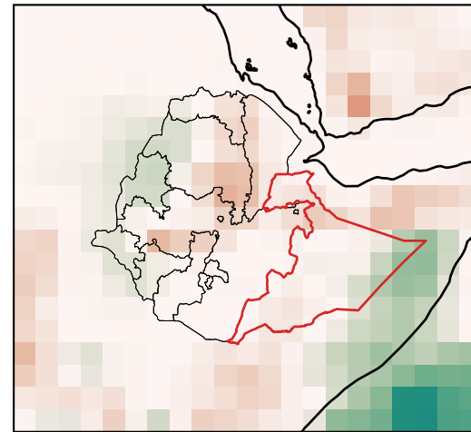
2000 MAM rainfall vs. 20% trigger threshold
