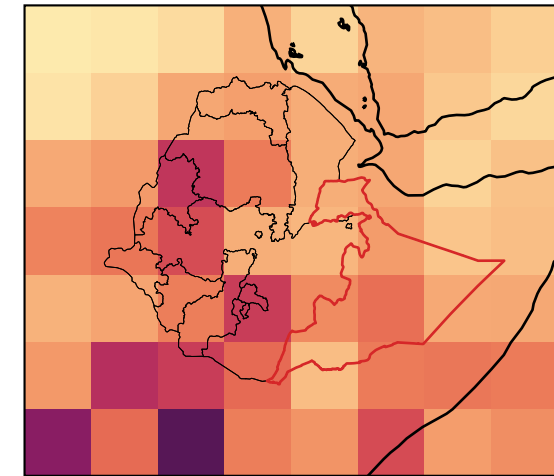
95% bootstrap IQR of trigger threshold
