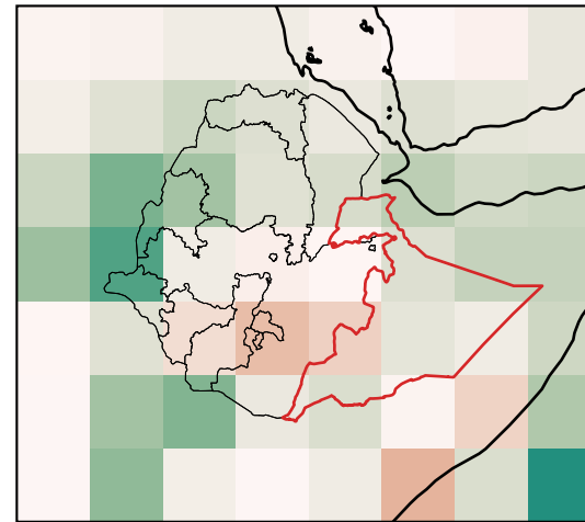
2021 MAM rainfall vs. 20% trigger threshold
