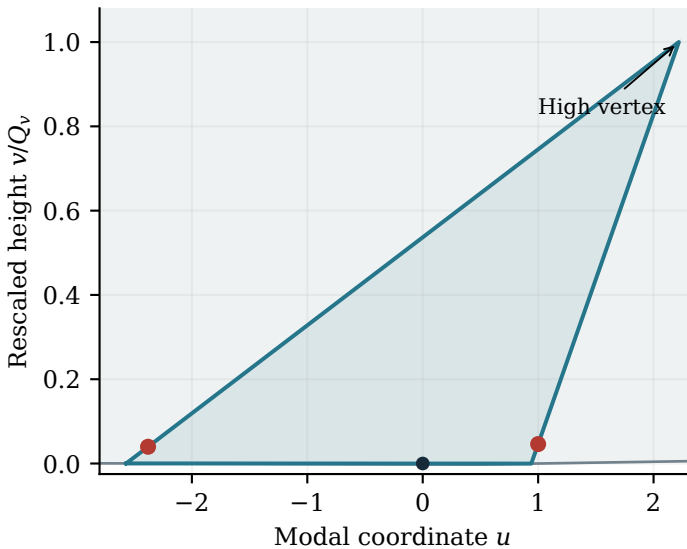
(a) Critical invariant triangle
