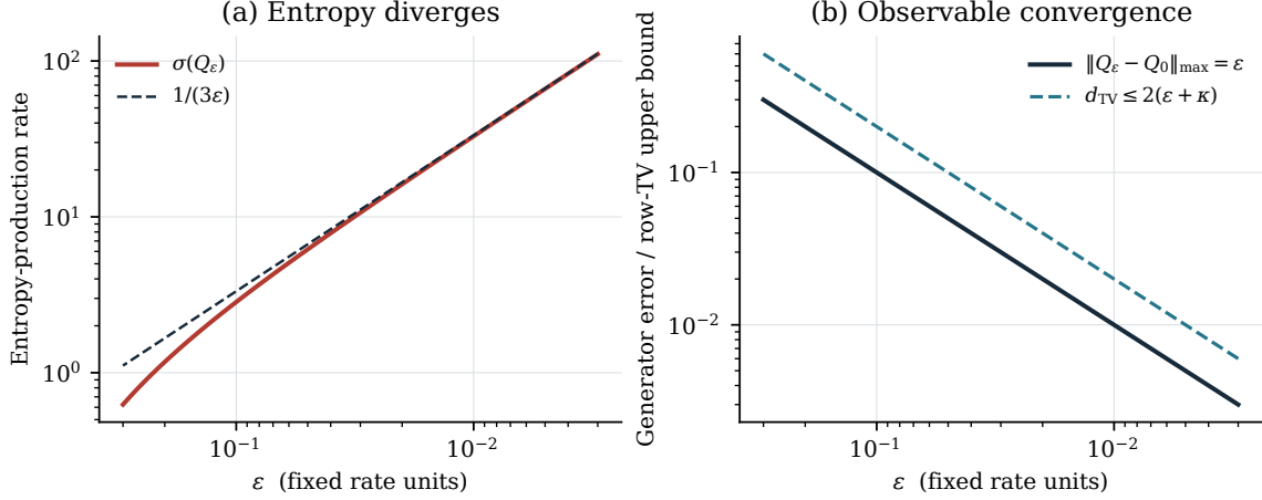
FIG. 2. The deterministic family (26) with k = \exp(-1/e^2) ; the figure uses \epsilon = e and \kappa = k . The rates converge to the unit tree and the analytic row-TV upper bound 2(e + k) tends to zero, while entropy diverges with asymptote 1/(3e) . The plotted TV line is a bound, not a measured distance. All finite-parameter models retain strictly positive reverse rates, observed rates one, trace -4 , and off-diagonal rates at most one. Arbitrary-precision evaluation avoids replacing the small reverse rate by zero.
