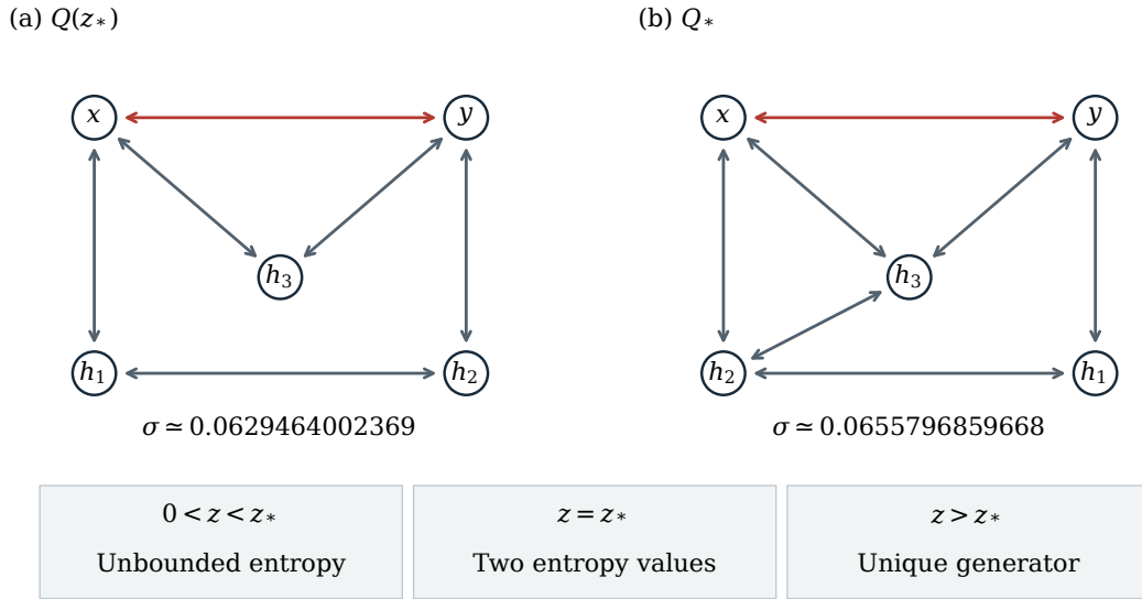
FIG. 4. Entropy-set properties for the family (61) under a five-state cap. Below the threshold the strip asserts unboundedness, not a complete range characterization. At the algebraic threshold the source and the connected-hidden alternative are the only physical realizations up to hidden labels. Paired arrows denote reciprocal support, not equal rates; only x \leftrightarrow y is observed. Entropy values in the figure are rounded; Eqs. (63)–(64) give certified intervals.
