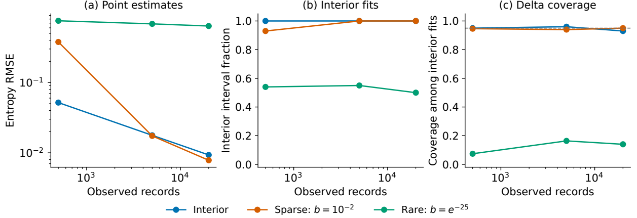
FIG. 3. Constructive inference and its failure near a sparse boundary. Each point uses 100 actual CTMC trajectories with the parameters in Table III. (a) Entropy RMSE includes boundary fits. (b) Fraction of fits permitting an interior delta calculation. (c) Raw interval coverage conditional on those fits, before the extra rare-mark warning; the dashed line is 95%. The rare-reverse case is poorly calibrated even after numerical boundary exclusion. The machine-readable output includes bias, variance, Wilson coverage intervals, all fitted rates, event counts, optimization statuses, and deterministic seeds.
