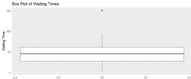
Boxplot for the waiting time data set
