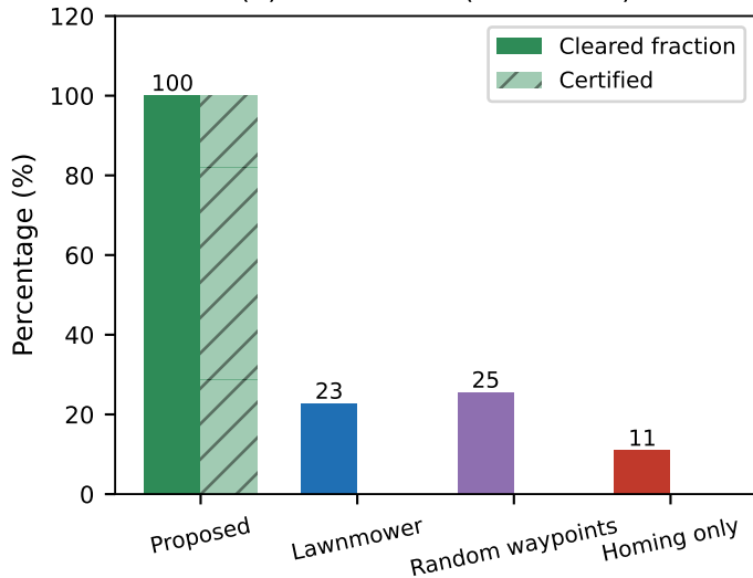
(b) Scenario S2 (directional)
