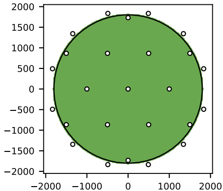
(b) Two-layer dense, 25 points detectable fraction = 1.000
