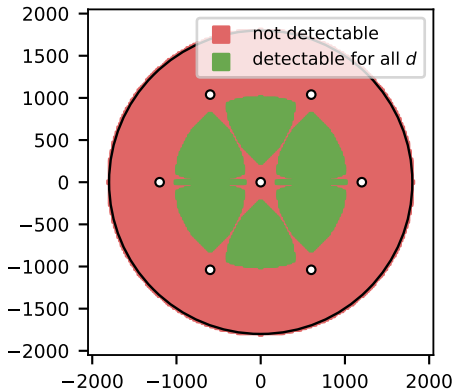
(a) Single-layer ring, 7 points detectable fraction = 0.236
