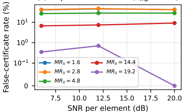
(c) Dependence on SNR ( \Gamma_{\text{mp}} = 7 dB)
