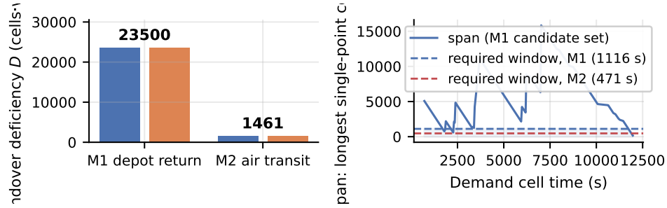
Figure 11: Co-design feedback loop. Panel (a): the handover deficiency is identical before and after re-optimising the departure instants, and the returned vector is the baseline vector (no shift survives as the incumbent), so on this frozen plan the departure instants are not where the residual deficiency can be removed. Panel (b): the span profile — the longest interval over which one single hover point can carry the whole demand — repeatedly falls below the required blackout window (dashed lines), which is the mechanism behind the obstruction.
