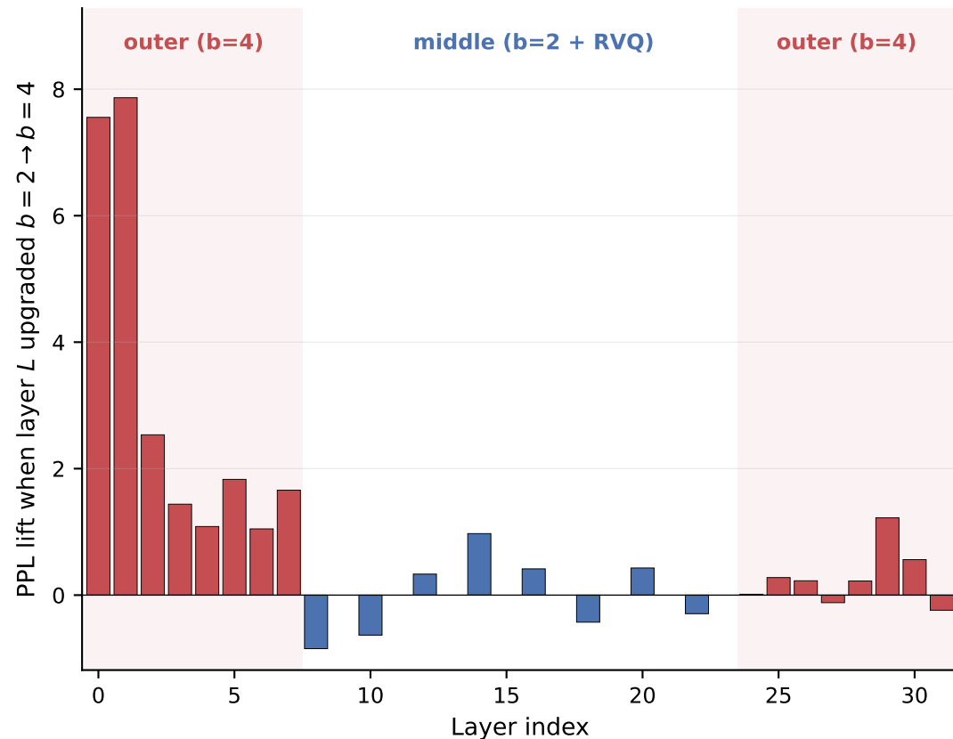
(b) R1-Distill-Llama-8B — boundary-to-middle ratio = 787
