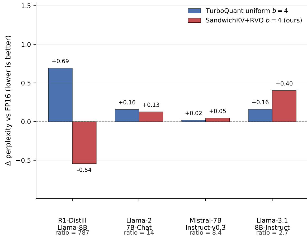
(a) Joint K+V at 4 bits/coord — multi-model comparison
