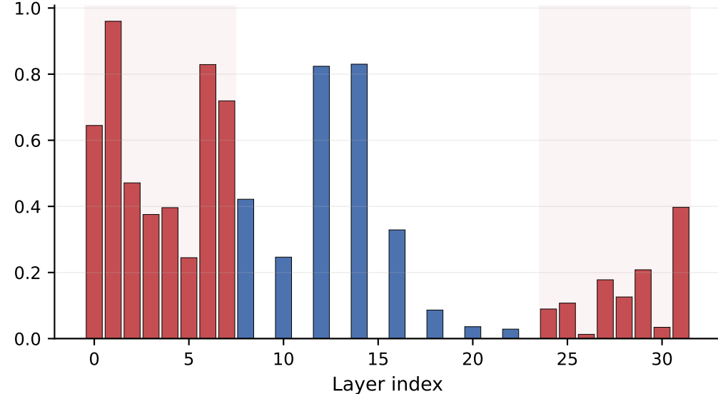
Llama-3.1 8B-Instruct ratio = 2.7 (flat)
