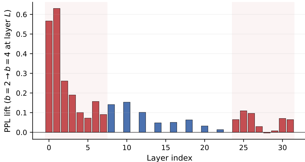
Mistral-7B Instruct-v0.3 ratio = 8.4 (boundary-dominant)
