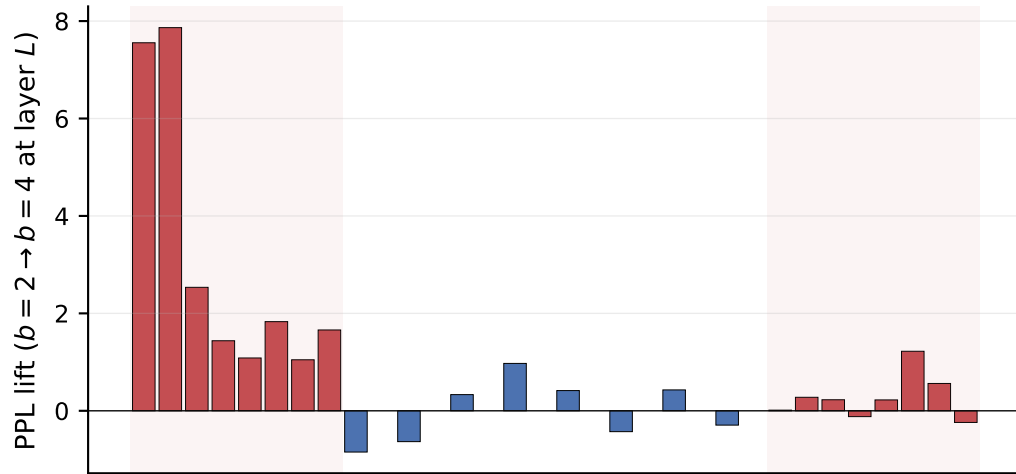
Mistral-7B Instruct-v0.3 ratio = 8.4 (boundary-dominant)
