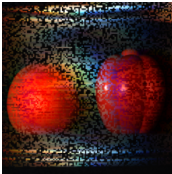
witness u \|Au - y_t\|/\|y_t\| = 1e-16
