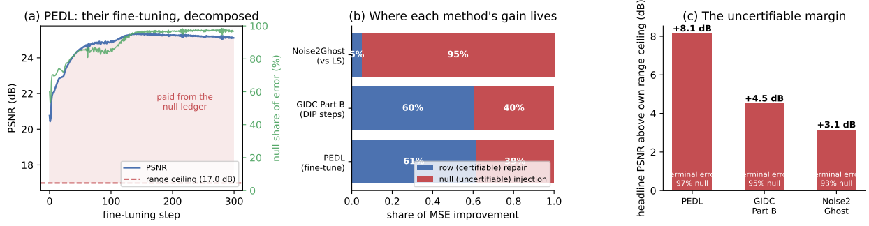
Figure 4: Fig. 4. Forensic decomposition of three published ghost-imaging pipelines on their own operators. (a) A fine-tuning trajectory decomposed per step: the PSNR rises past the operator’s range ceiling, and everything above it is supplied from the null space. (b) Attribution of each method’s improvement into row-space repair and null-space supply. (c) Every reported result stands +3.1 to +8.1 dB above its own range ceiling, with terminal error 93–97% null. GI: ghost imaging; P_Rx : oracle row-space (measured) image; P_0 : unmeasured subspace; PSNR: peak signal-to-noise ratio.
