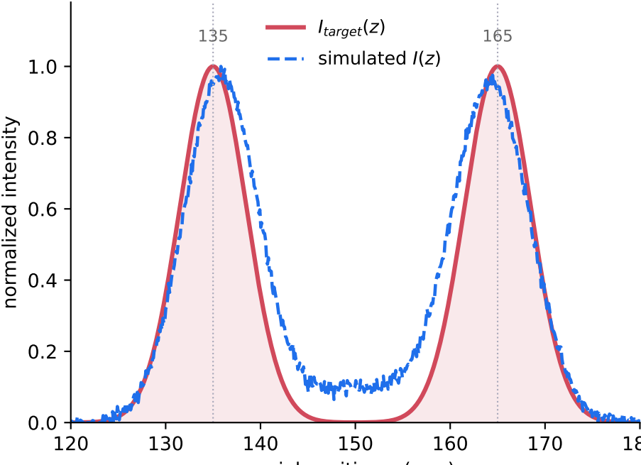
(a) Target vs. simulated axial intensity
