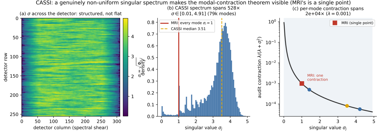
Figure 4: Fig. 5. The per-mode contraction on a real coded aperture. Left, the singular value \sigma_j = \sqrt{\Phi_s} across the detector plane. Middle, the distribution of \sigma_j over 79,360 measured modes spans a 528\times range; the red line marks the single value ( \sigma = 1 ) of a flat-spectrum masked-Fourier operator. Right, the per-mode audit factor \lambda/(\lambda + \sigma_j^2) spreads across four orders of magnitude, where a flat-spectrum operator collapses to a single point.
