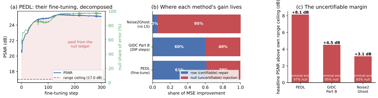
Figure 3: Fig. 4. Forensic decomposition of three published ghost-imaging pipelines on their own operators. (a) A fine-tuning trajectory decomposed per step: the PSNR rises past the operator’s range ceiling, and everything above it is supplied from the null space. (b) Attribution of each method’s improvement into row-space repair and null-space supply. (c) Every reported result stands +3.1 to +8.1 dB above its own range ceiling, with terminal error 93–97% null. GI: ghost imaging.
