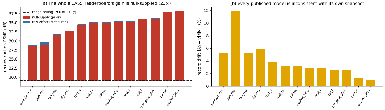
Figure 5: Fig. 6. Reported spectral-imaging gains decomposed on the shared real coded aperture. (a) Thirteen published models against the 19.04 dB min-norm range ceiling; twelve of the thirteen gains are 100–101% null-supplied (one exception at 93%), and the row-space effect is slightly negative. (b) Each model’s record inconsistency \|A\hat{x} - y\|/\|y\| ranges from 0.9% to 12%.
