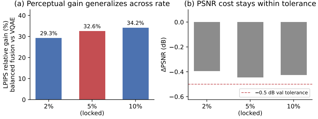
Figure 6: the perceptual gain generalizes across sampling rate (development-level) . Balanced fusion’s relative LPIPS gain over the VQAE branch at 2%, 5% (locked), and 10% sampling, with the PSNR cost within the pre-registered -0.5 dB validation tolerance at every rate (3 seeds per rate, all same-direction).
