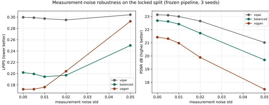
Figure 7: the recommended dial position is also the robust one (development-level) . LPIPS versus bucket-noise level for the VQAE branch, balanced fusion, and full VQGAN with B frozen: full VQGAN’s synthesized fine detail amplifies measurement noise and degrades sharply, while balanced fusion overtakes it at \sigma_\epsilon = 0.02 and degrades gracefully; the exact consistency A\hat{x}_B = y concerns the row space at every noise level and is unaffected.
