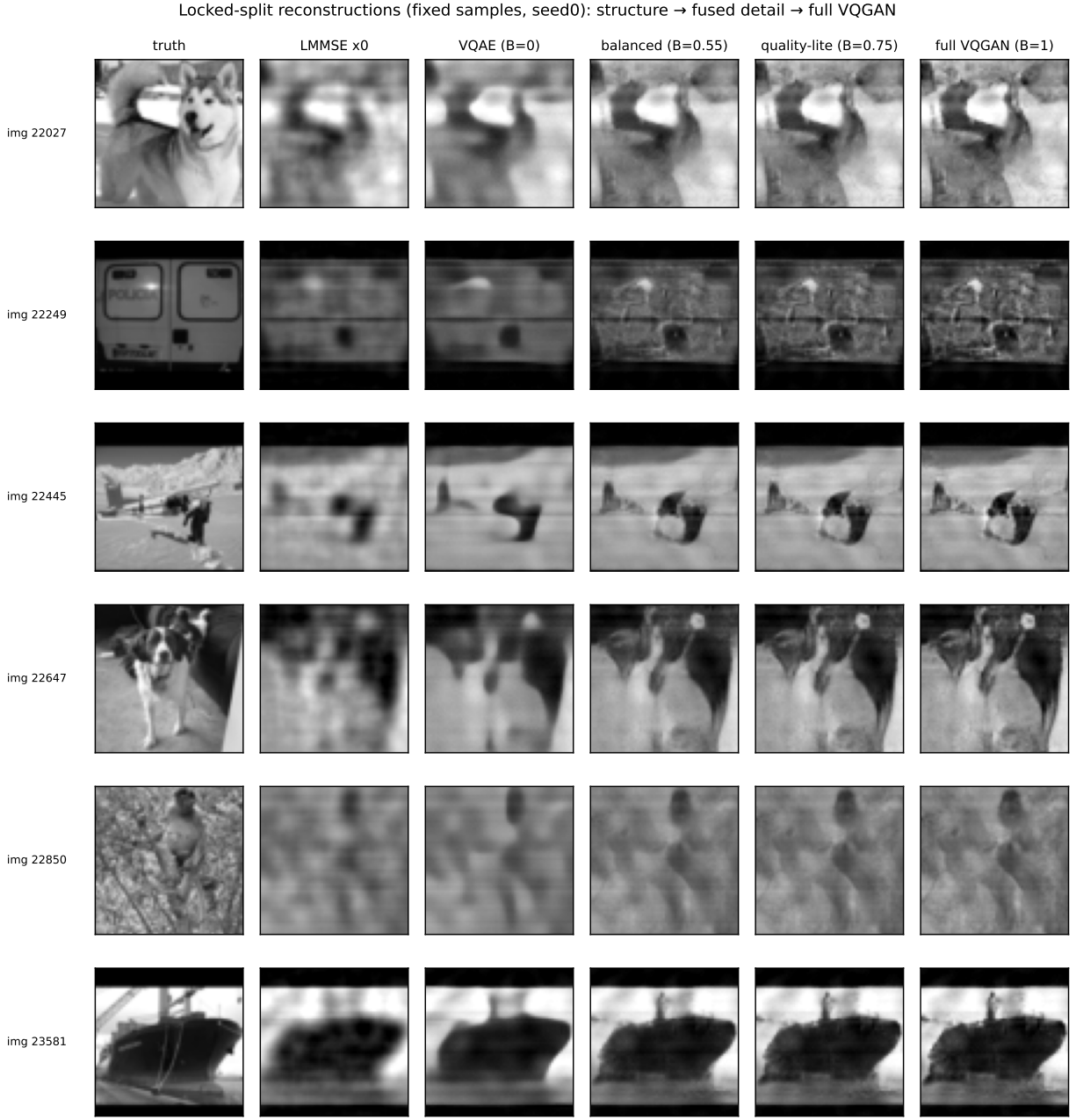
Figure 5: locked-split reconstructions at the named operating points. Fixed samples reconstructed by the LMMSE anchor, the VQAE branch, balanced fusion, quality-lite, and full VQGAN, against ground truth. Moving right along the dial adds perceptual detail — sharper texture, more natural spectra — while every column reproduces the identical bucket record exactly; the added detail lives entirely in the null space the measurement cannot see.
