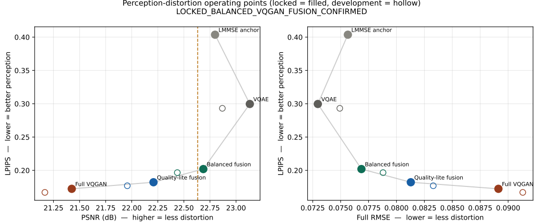
Figure 3: the metered perception–distortion ladder. Named operating points of Table 1 on the perception–distortion plane (LPIPS versus PSNR/RMSE): the LMMSE anchor, the VQAE structure branch ( B=0 ), the pre-registered balanced point ( B\approx 0.55 ), quality-lite ( B\approx 0.72 ), and full VQGAN ( B=1 ). The ladder is monotone — perceptual quality is bought at a metered pixel-fidelity cost — and every point satisfies A\hat{x} = y to \text{RelMeasErr} \sim 10^{-7} ; the trade moves entirely within the null space.
