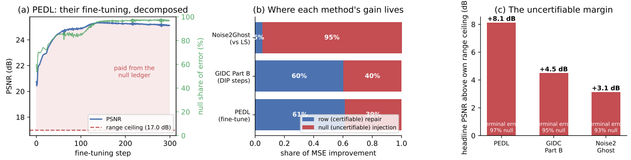
Figure 8: projector forensics of three published DL-GI pipelines, on their own operators. (a) The fine-tuning trajectory of the physics-enhanced pipeline (Wang et al. 2022a), decomposed per step: PSNR rises past the operator’s range ceiling (dashed) — everything above it is paid from the null ledger — while the null share of the remaining error climbs to 96.9%. (b) Attribution of each method’s MSE improvement: row-space (certifiable) repair versus null-space (uncertifiable) injection — 61/39 for fine-tuning, 60/40 for GIDC’s untrained DIP on real measured speckle, 5/95 for Noise2Ghost against least squares on a noisy record. (c) Every headline PSNR stands +3.1 to +8.1 dB above its own operator’s range ceiling, with terminal error 93–97% null.
