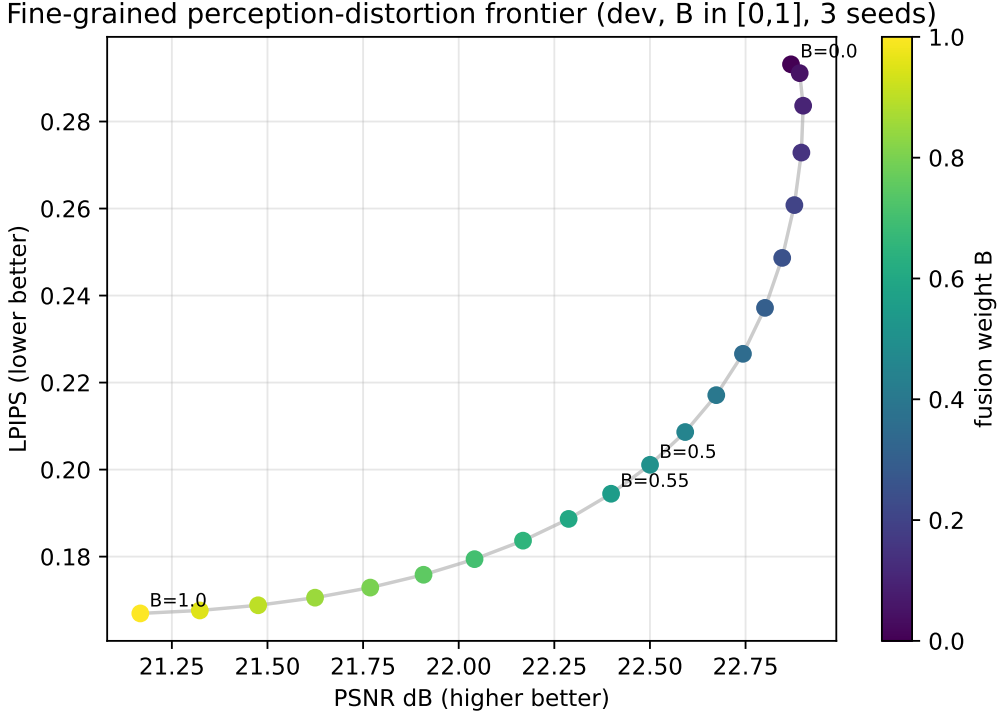
Figure 4: the frontier is smooth, monotone, and interior-optimum-free. A dense 21-point development-split sweep of the fusion weight B (step 0.05): LPIPS falls strictly monotonically from 0.293 to 0.167 while PSNR declines from 22.87 to 21.17 dB (one shallow interior maximum of +0.03 dB at B = 0.10 ). No discontinuity and no interior perceptual optimum — the dial is a stable interpolation, not a fragile hyperparameter.
