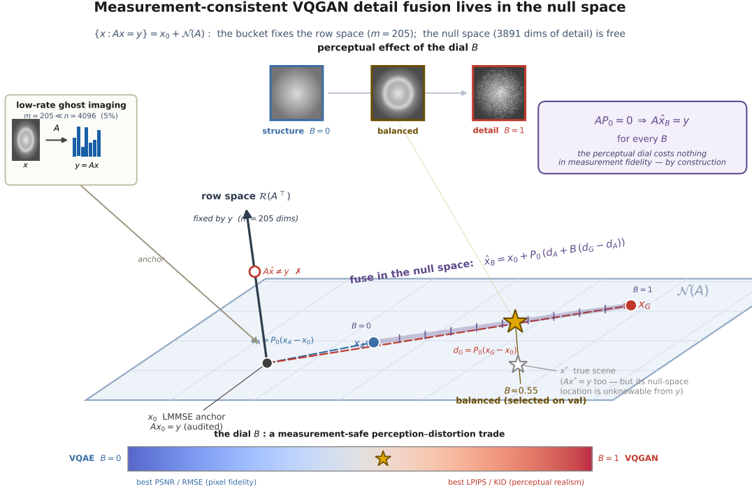
Figure 2: the mechanism. Every measurement-consistent image lies on the affine flat \{x : Ax = y\} = x_0 + \mathcal{N}(A) ; the bucket fixes only the orthogonal row-space direction, so leaving the flat changes y . From the measurement-audited LMMSE anchor x_0 , the fusion weight B slides the reconstruction along the in-plane dial from the VQAE structure point ( B=0 ) to the VQGAN detail point ( B=1 ). Because AP_0 = 0 , every B stays on the flat and A\hat{x}_B = y holds exactly. The true scene x^* also lies on the flat, but its null-space location is unknowable from y — the same geometry read as barrier and as license.
