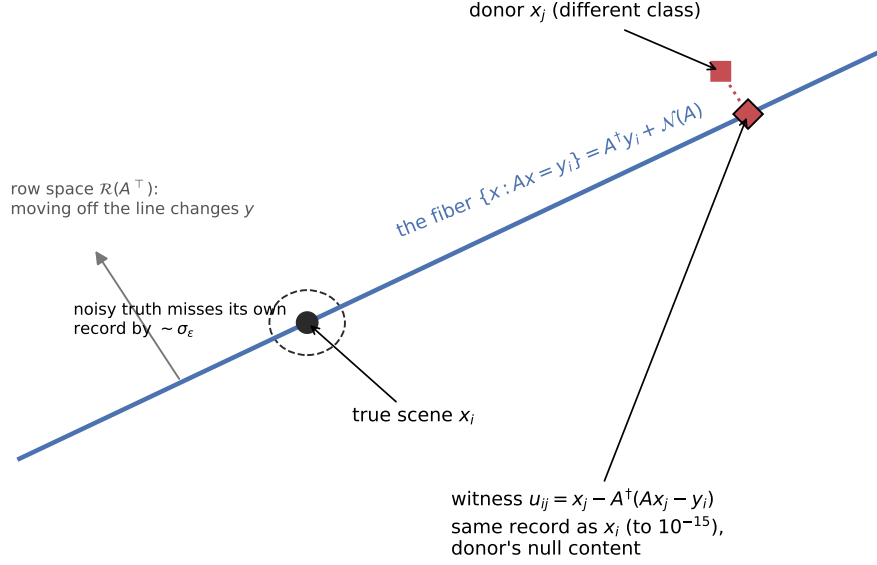
Figure 2: The converse in one picture. Every point on the line (the fiber \{x : Ax = y_i\} ) reproduces the record; moving off the line is the only thing the measurement can see. The witness is the donor projected onto the fiber: it matches the record to 10^{-15} — more tightly than the noisy truth (dashed circle, radius \sim \sigma_\epsilon ) matches its own record — while carrying the donor’s null content.
