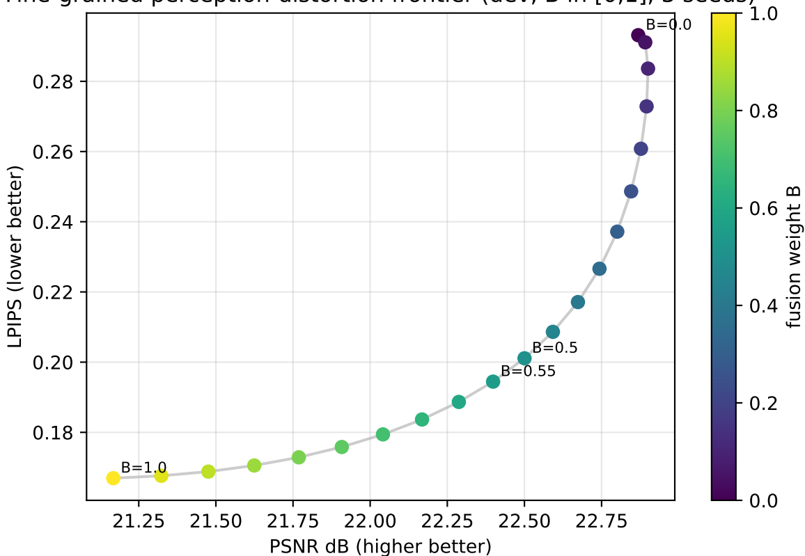
Fine-grained perception-distortion frontier (dev, B in [0,1], 3 seeds)
