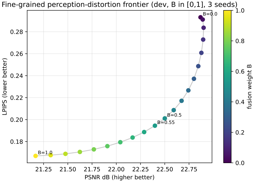
Figure 8: The dense 21-point sweep of the dial: LPIPS strictly monotone from 0.293 to 0.167; PSNR declines from 22.87 to 21.17 dB with one shallow interior maximum (+0.03 dB at B = 0.10 ).
