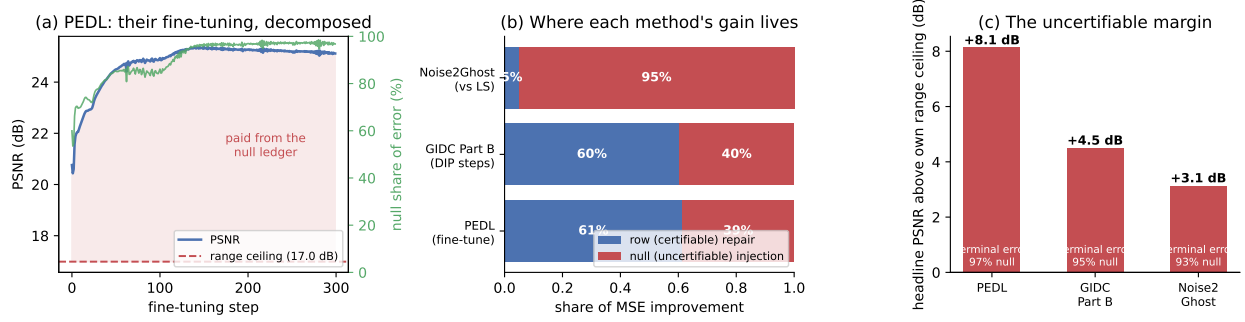
Figure 7: Three paradigms, three operators, one structure. (a) The fine-tuning trajectory decomposed per step: PSNR rises past the operator’s range ceiling — everything above it is paid from the null ledger. (b) Attribution of each method’s improvement: row repair vs null injection. (c) Every headline stands +3.1 to +8.1 dB above its own range ceiling with terminal error 93–97% null.
