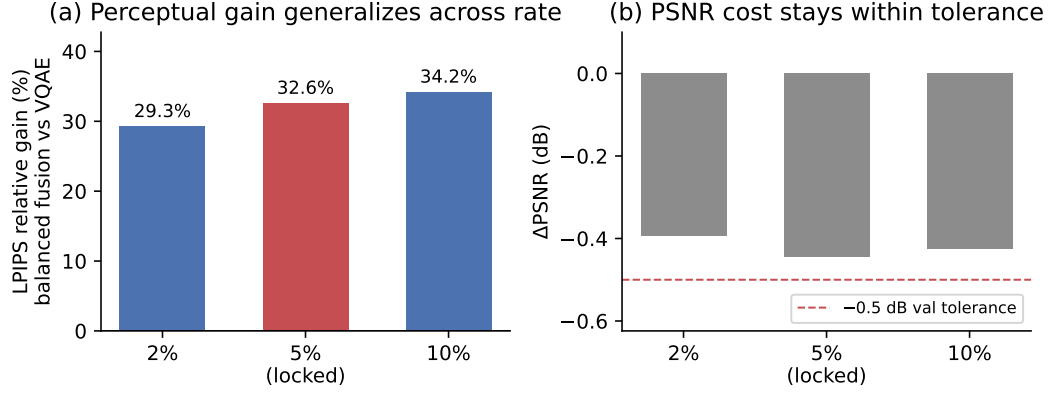
Figure 9: Cross-rate generalization (development-level): the balanced dial’s relative LPIPS gain at 2%, 5% (locked), and 10% sampling.
