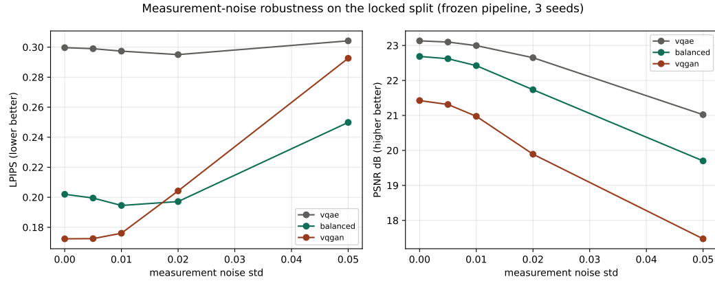
Figure 10: Noise robustness (development-level): balanced fusion degrades gracefully and overtakes full VQGAN at \sigma_\varepsilon = 0.02 .
