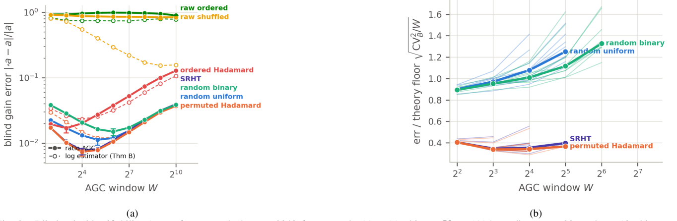
Fig. 3. Blind gain identifiability (seven frame-matched arms, 2048 frames each; 32 \times 32 objects, K = 1024 ; medians over 20 seeds \times 10 objects at \rho_{\text{pair}} = 10^{-3} , s = 0.1 ). (a) Blind gain error \|\hat{a} - a\|/\|a\| versus window W under the ratio AGC (solid, filled) and the Theorem-B log estimator on the R > 0 record (dashed, open); raw signed-Walsh arms are diagnostic-only. Error bars: two-way clustered 95% CIs of the median best-window error. (b) Errors normalized by the theory floor \sqrt{CV_B^2/W} collapse across the ten objects. Quantitative values: Sec. 9.2 and Table III.
