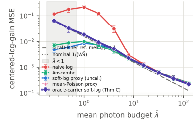
Fig. 5. Low-photon robustness under Poisson counting, on identical random-basis carriers and shared gain traces (soft-log \alpha = 0.5 , W = 64 , \rho_{\text{pair}} = 10^{-3} , s = 0.1 ; truncated edge windows). Centered-log-gain MSE (Theorem C’s log-domain loss, Fisher-comparable at d = 0 ) versus \bar{\lambda} against the local realized Fisher reference \text{mean}_n[1/I_n] , I_n = \sum_{k \in W_n} \lambda_k (dashed; dotted: nominal 1/(W\bar{\lambda}) ; shaded: \bar{\lambda} < 1 ). The oracle-known-carrier calibrated soft-log of Theorem C (diamonds; oracle carriers) is the only arm tracking the 1/(W\bar{\lambda}) law and stays above the Fisher reference at every tested budget (the mean-Poisson proxy overlaps it); the uncalibrated proxy and Anscombe buy low-count MSE with shrinkage bias (sub-Fisher at \bar{\lambda} \leq 2 ). Ratios, slopes, drift-limited floor: Sec. 9.5.
