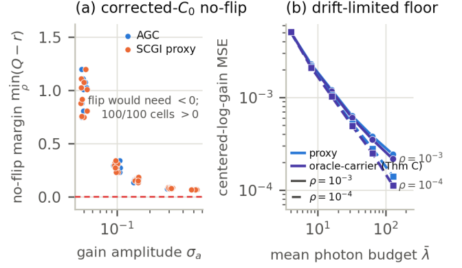
Fig. 12. Extended flip-boundary detail and the low-photon floor probe. (a) Corrected- C_0 no-flip margins for the blind random+DGI arm: per-cell minimum over the drift grid of Q - r for the conditional scalar proxy with drift-leverage constant 1 + C_0^{\text{lev,raw}} background, for the AGC and SCGI-proxy corrections; a flip would require a negative value, and all 100/100 cells are positive, matching the empirical no-flip outcome of Sec. 9.4. This is a consistency check, not a same-record scalar theorem validation. (b) High-photon floor probe: log-domain gain MSE versus mean photon budget \bar{\lambda} for the uncalibrated proxy and the oracle-known-carrier calibrated soft-log (Theorem C) at \rho = 10^{-3} (solid) and \rho = 10^{-4} (dashed); the two drift rates share the photon-limited regime and separate only at the floor ( 2.434 \times 10^{-4} versus 1.411 \times 10^{-4} for the proxy, 2.168 \times 10^{-4} versus 1.125 \times 10^{-4} for the oracle-carrier arm — 10.92% lower at \rho = 10^{-3} , 20.28% lower at \rho = 10^{-4} ), which is therefore drift-limited, not photon-limited.
