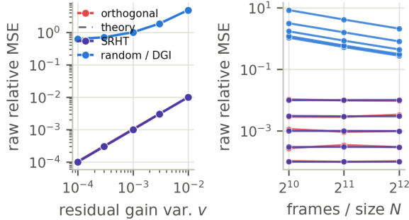
Fig. 9. Reconstruction bridge in total raw relative MSE (8100 rows: three reconstructors, N \in \{1024, 2048, 4096\} , six v levels including the v = 0 baseline, ten objects, fifteen seeds). Markers: measured R_{\text{raw}} ; dashed: fixed-design prediction R_{\text{raw}}^{\text{raw}} + B_L v . Deterministic inverses are flat in N ; random/DGI follows 1/N . Exact leverage, ratios, and identity residual: main-text Sec. 9.3.
