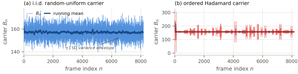
Fig. 2. Carrier stationarity: noiseless bucket carriers B_n (thin), running means (bold), and the \pm 1 SD envelope for one object (digit_0; 8192 frames, 64 \times 64 ), before any gain is applied. (a) The i.i.d. random-uniform carrier is a flat, object-independent noise band; (b) the ordered Hadamard trace is the object's coefficient envelope — a deterministic, non-stationary temporal signature. Rejection counts and the Parseval invariant: Sec. 9.1.
