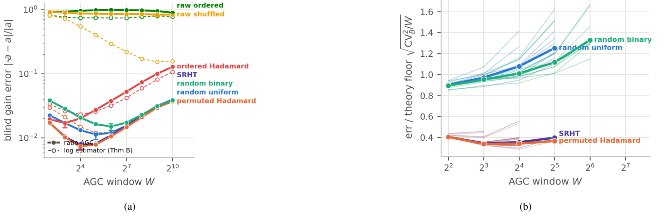
Fig. 3. Blind gain identifiability (seven frame-matched arms, 2048 frames each; 32 \times 32 objects, K = 1024 ; medians over 20 \text{ seeds} \times 10 \text{ objects} at \rho_{\text{pair}} = 10^{-3} , s = 0.1 ). (a) Blind gain error \|\hat{a} - a\|/\|a\| versus window W under the ratio AGC (solid, filled) and the Theorem-B log estimator on the R > 0 record (dashed, open); raw signed-Walsh arms are diagnostic-only. Error bars: two-way clustered 95% CIs of the median best-window error. (b) Errors normalized by the theory floor \sqrt{CV_B^2/W} collapse across the ten objects. Quantitative values: Sec. 9.2 and Table S2.
