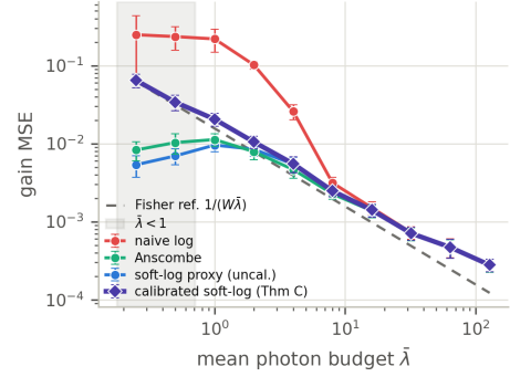
Fig. 5. Low-photon robustness under Poisson counting, on identical random-basis carriers and shared gain traces (soft-log \alpha = 0.5 , W = 64 , \rho_{\text{pair}} = 10^{-3} , s = 0.1 ; four estimator arms per paired Poisson draw). Gain MSE versus \bar{\lambda} against the local Fisher reference 1/(W\bar{\lambda}) (dashed; shaded: \bar{\lambda} < 1 shrinkage-bias region). The calibrated soft-log of Theorem C (diamonds) is the only arm tracking the 1/(W\bar{\lambda}) law and is never sub-Fisher; the proxy and Anscombe buy low-count MSE with shrinkage bias. Ratios, slopes, and the drift-limited floor: Sec. 9.5.
