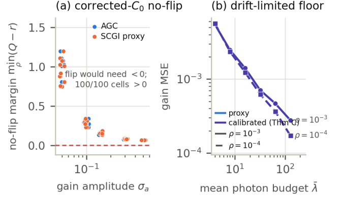
Fig. S6. Extended flip-boundary detail and the low-photon floor probe. (a) Corrected- C_0 no-flip margins for the blind random+DGI arm: per-cell minimum over the drift grid of Q - r (the flip criterion of Prop 3 with drift-leverage constant 1 + C_0^{\text{raw}} ), for the AGC and SCGI-proxy corrections; a flip would require a negative value, and all 100/100 cells are positive, matching the no-flip outcome of Sec. 9.4. (b) High-photon floor probe: gain MSE versus mean photon budget \bar{\lambda} for the uncalibrated proxy and the calibrated soft-log (Theorem C) at \rho = 10^{-3} (solid) and \rho = 10^{-4} (dashed); the two drift rates share the photon-limited regime and separate only at the floor ( 2.78 \times 10^{-4} versus 1.73 \times 10^{-4} ), which is therefore drift-limited, not photon-limited.
