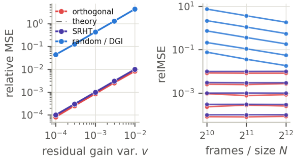
Fig. S3. Reconstruction bridge (Theorem 1 tested as an identity, on a balanced 8100-row design: three reconstructors, N \in \{1024, 2048, 4096\} , six injected residual-gain variances v , ten objects, fifteen seeds; moved from the main document). Predicted versus measured scale-aligned relMSE: the deterministic inverses are flat in N , as B_L = 1 demands, while the random/DGI arm decays as 1/N at every v with a quantitative leverage law. Slopes, leverage values, and the DC-dominated alignment effect: main-text Sec. 9.3.
