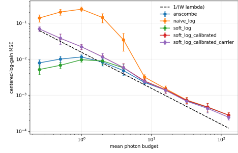
Fig. 5. Low-photon robustness under Poisson counting, on identical random-basis carriers and shared gain traces (soft-log \alpha = 0.5 , W = 64 , \rho_{\text{pair}} = 10^{-3} , s = 0.1 ; four estimator arms per paired Poisson draw). Centered-log-gain MSE (Theorem C’s log-domain loss, the only metric comparable to the log-intensity Poisson information) versus \bar{\lambda} against the local Fisher reference 1/(W\bar{\lambda}) (dashed; shaded: \bar{\lambda} < 1 shrinkage-bias region). The carrier-aware calibrated soft-log of Theorem C (diamonds) is the only arm tracking the 1/(W\bar{\lambda}) law and stays above the Fisher reference at every tested budget; the uncalibrated proxy and Anscombe buy low-count MSE with shrinkage bias (sub-Fisher at \bar{\lambda} \leq 1 ). Ratios, slopes, and the drift-limited floor: Sec. 9.5.
