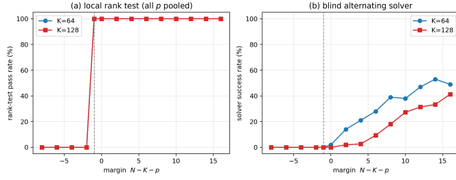
Fig. 8. Tall-design threshold scan (a direct test of Theorem A’s counting) at K = 64 (20 seeds/cell, 1300 cells) and K = 128 (30 seeds/cell, 1950 cells), over five low-pass drift dimensions p \in \{3, 5, 9, 17, 33\} with margins N - K - p \in [-8, +16] , all p pooled. (a) The local rank test on the collision Jacobian transitions from 0% to 100% pass exactly at margin N - K - p = -1 for every p at both sizes (3250 cells, no exceptions), verifying the local differential threshold N = K + p - 1 . (b) The companion blind alternating solver (8 restarts \times 150 iterations) starts at the same wall but climbs slowly — about 2% success at margin 0 and only \sim 50\% at margin +16 for K = 64 ( \sim 41\% for K = 128 ) — an algorithmic-recovery observation, not a uniqueness test: uniqueness and recovery separate as Sec. 2’s third notion anticipates.
