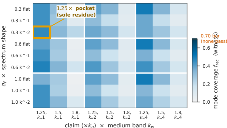
(c) 81-cell Fisher atlas: REGION_EMPTY, 0/81 pass
