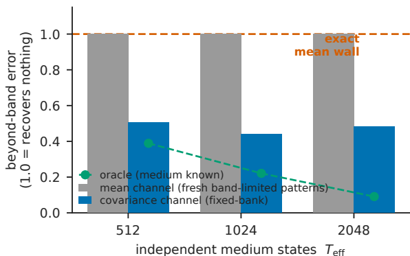
(a) spectral law: covariance crosses the mean wall
