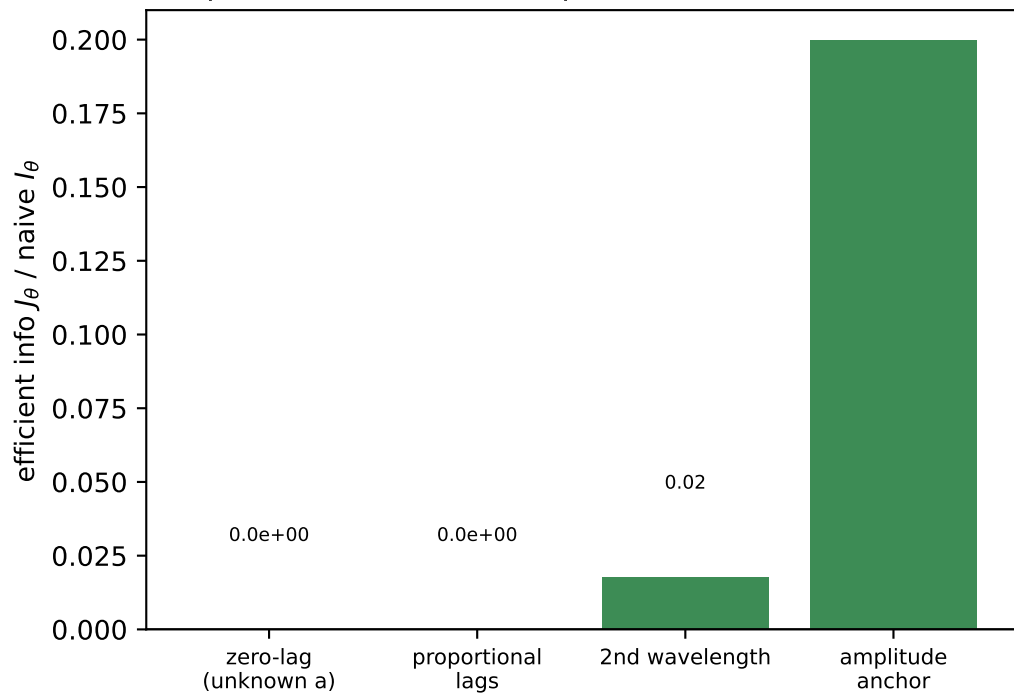
Bank B -- nuisance quotient: 0.20 amplitude confound collapses info, anchor restores it
