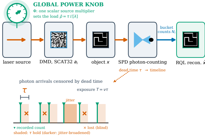
(a) Dead-time-aware single-pixel imaging pipeline
