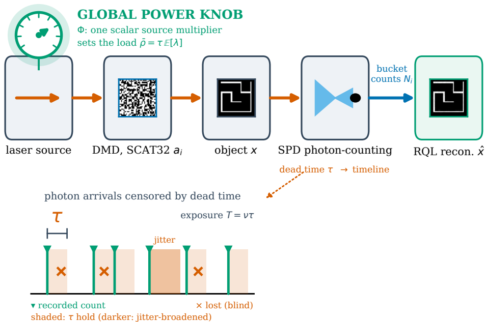
(a) Dead-time-aware single-pixel imaging pipeline
