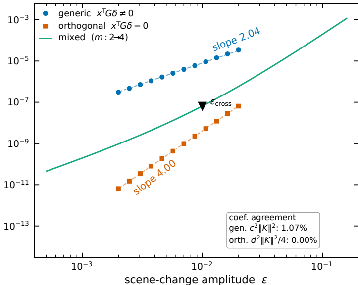
profiled Chernoff distance C_*(\varepsilon; \delta)
