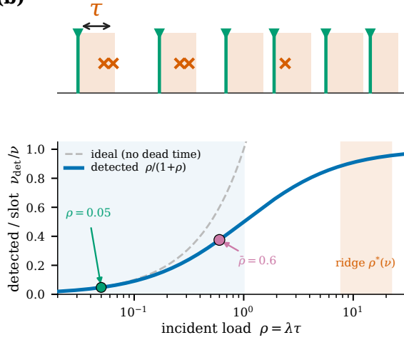
Figure 1: Contrast–dead-time operating map for high-flux single-pixel imaging. DMD: digital micromirror device; SPD: single-pixel (bucket) photon-counting detector; RQL: renewal quasi-likelihood reconstruction; a_i : binary illumination pattern; x : scene; N_i : integrated bucket count; \hat{x} : reconstruction; \Phi : incident-flux scale; d : dark rate; \tau : detector dead time; \rho = \lambda\tau : per-slot detector load; \nu = T/\tau : dead-time slots per exposure T ; C_u = \text{sd}_i(u_i)/\text{mean}_i(u_i) : measured bucket-energy contrast of u_i = a_i^\top x ; \Gamma = C_u \sqrt{\nu\rho/(1+\rho)} : contrast-to-count-noise index. (a) Single-pixel imaging chain: structured illumination from a DMD probes a low- or high-contrast scene x , and the bucket counts N_i feed the RQL reconstruction \hat{x} under the forward model \lambda_i = \Phi a_i^\top x + d , exposure T = \nu\tau . (b) Dead-time mechanism: after each registered count the detector is blind for \tau (shaded), censoring later arrivals ( \times ); the mean detected counts per slot \nu_{\text{det}}/\nu = \rho/(1+\rho) bend away from the ideal (dashed) as the load rises, while the exact count-information peaks on the ridge \rho^*(\nu) = (6\nu)^{1/3} - 2/3 ( \rho^* \approx 7.8 and 22.2 at \nu = 100 and 2000 , respectively), well beyond the conventional \rho = 0.05 and the high-flux \bar{\rho} = 0.6 operating points. (c) Operating map in the contrast–load plane: the photon-limited onset \Gamma = 1 is a descriptive photon-limited-onset proxy, marking bucket modulation comparable to count noise; it is not a predicted or validated boundary for high-flux image benefit. The six Study-2 structural families are placed at the high-flux operating load \bar{\rho} = 0.6 by their measured bucket contrast and coloured by the frozen acquisition-speed gate outcome, with the number of accelerating instances shown as a green wedge: maze ( C_u = 0.53 ), glyph (0.41) and spokes (0.38) accelerate 4/4, chirp (0.28) 3/4, contour (0.27) 1/4, and microtexture (0.17) 0/4, respectively, while the dense k = 512 rung ( C_u = 0.040 ) sits at the \Gamma = 1 multiplex-limited boundary. All six family markers share the single operating load \bar{\rho} = 0.6 ; the horizontal offsets are cosmetic, applied only to separate near-coincident markers (chirp and contour differ by 0.01 in C_u ), and thin leader lines tie each family label to its marker. The contrast-controlled transition band is descriptive and does not estimate a universal critical contrast. Grayscale object icons are for display purposes.
