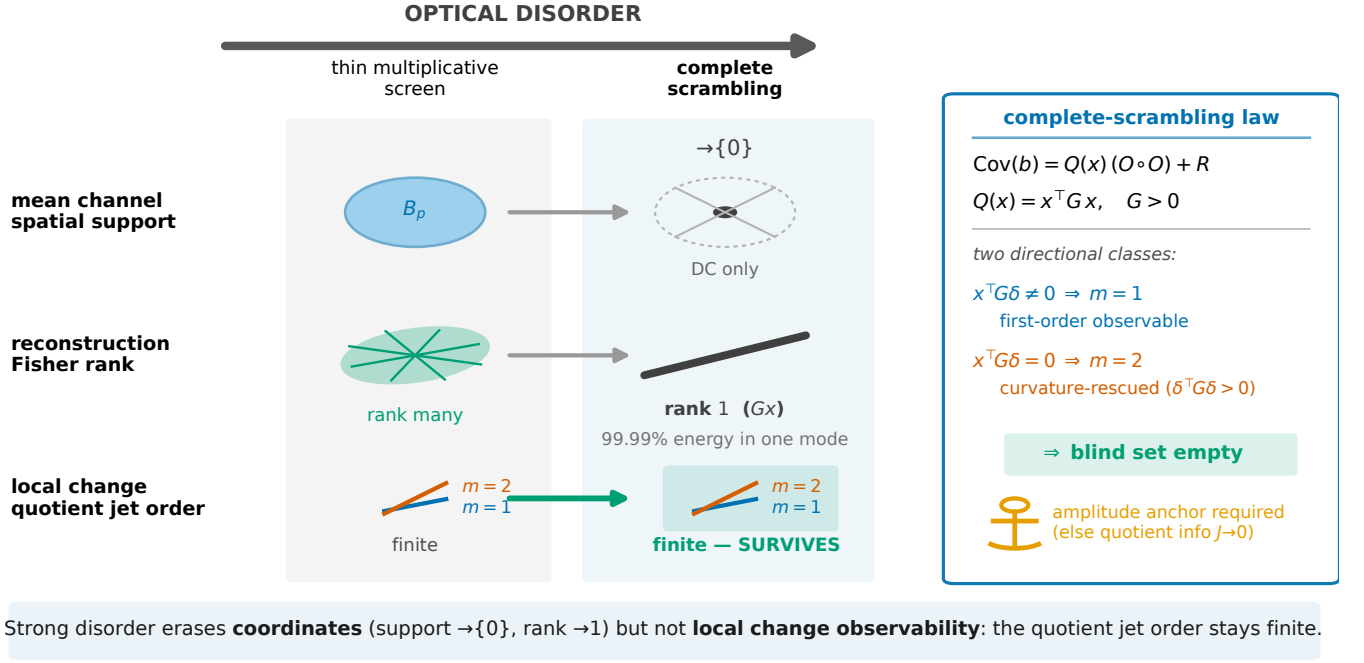
FIG. 1. Rank collapses; jets survive. As optical disorder grows from a thin multiplicative screen to complete scrambling, the mean-channel spatial support contracts B_p \rightarrow \{0\} (DC only) and the reconstruction Fisher rank collapses from many modes to one (99.99% of the covariance energy in the single direction Gx ), while the quotient jet order stays finite ( m = 1 or 2 ) and the local blind set stays empty. At the scrambling endpoint the record covariance factors as \text{Cov}(b) = Q(x) (O \circ O) + R with Q = x^\top G x , and the two directional classes u = 2x^\top G \delta , v = 2\delta^\top G \delta set the contact order. The amplitude-anchor condition (icon) is a prerequisite, not a caveat: without it the quotient information vanishes.
