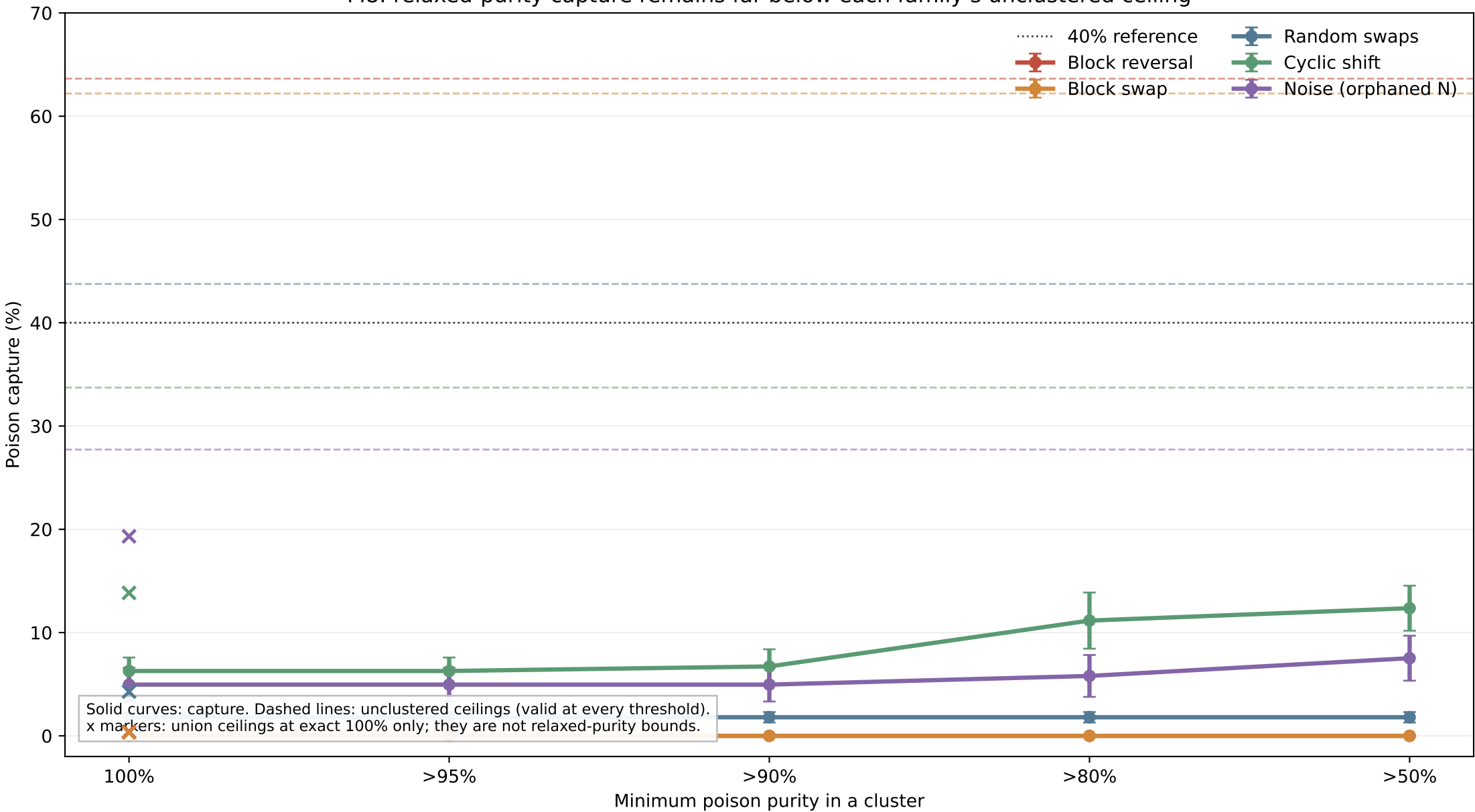
M8: relaxed-purity capture remains far below each family's unclustered ceiling
