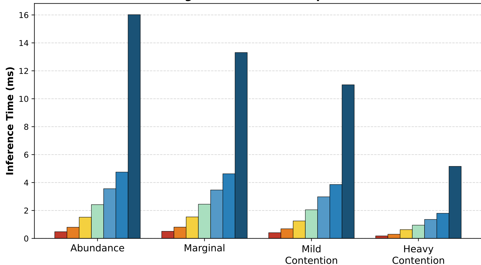
DRL Agent Inference Time per Task
