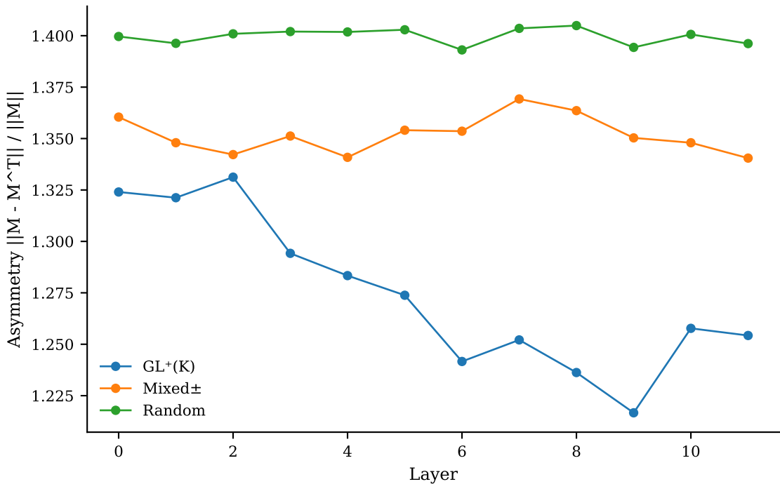
Gauge Structure: Asymmetry of W_Q W_K^T
