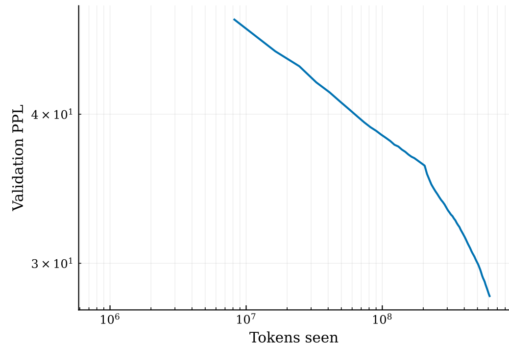
Training trajectory: PPL vs tokens seen
