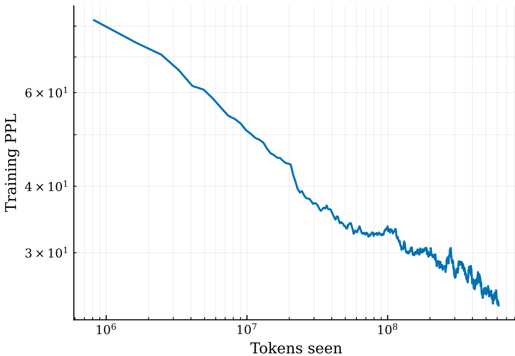
Training trajectory: PPL vs tokens seen
