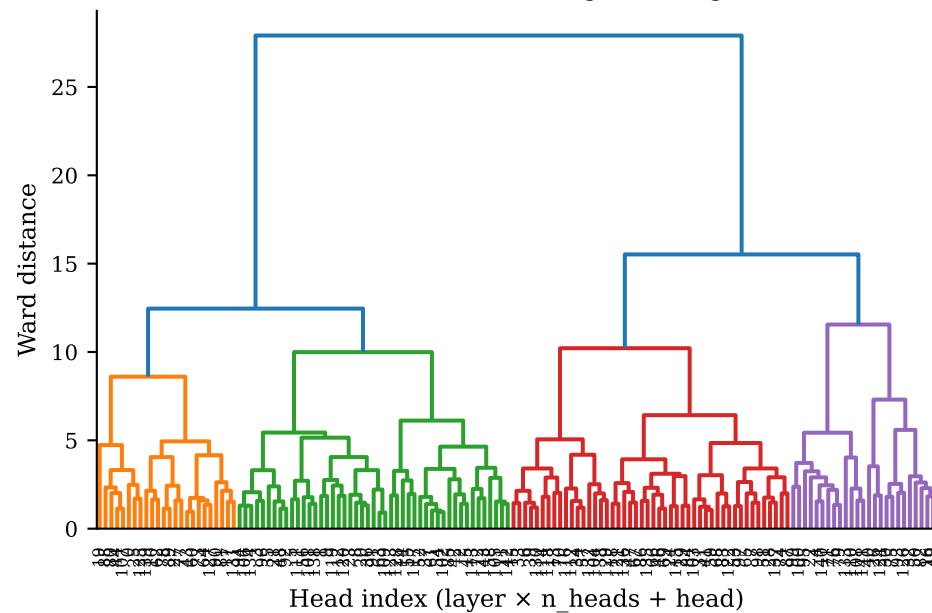
Mixed \pm : Cluster Assignment
