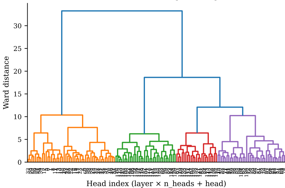
GL + (K): Cluster Assignment
