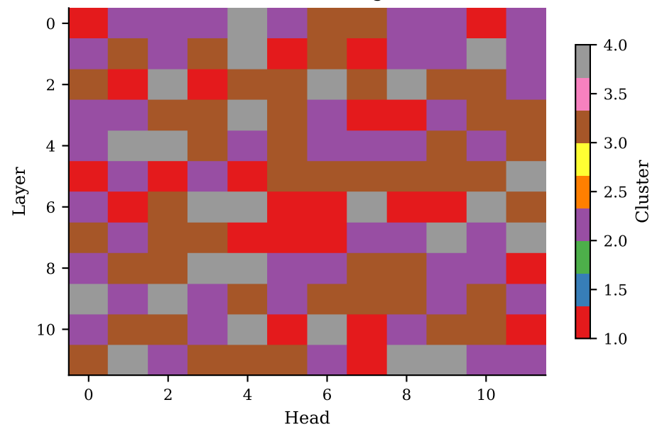
Mixed \pm : Cluster Assignment
