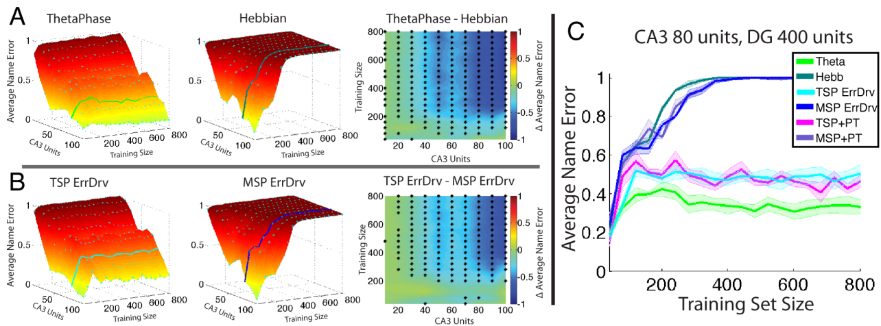
Figure 3. Comparison of network performance contrasting Hebbian and Error Driven learning rules. Network performance plotted across various network sizes and training set sizes. A ) Surface plots of the average Name Error across the full training set plotted on the left for both the theta-phase (i.e. error-driven learning in both MSP and TSP) and the Hebbian network, and the difference between theta-phase and Hebbian surfaces plotted on the right with an asterisk showing values significantly ( p < 0.005 ) different from 0. Cyan dots in the surface plots are data points where performance was measured. B ) Same Name Error surface plots with the left panel (labeled TSP ErrDrv) showing performance from a network with error-driven learning in the TSP and Hebbian learning in the MSP. Middle panel (labeled MSP ErrDrv) shows performance from a network with Hebbian learning in the TSP and error-driven learning in the MSP. Difference between these two shown on the right. C ) Plot of network performance taken from A and B for a single network size of 80 CA3 units and 400 DG units. Line color is shown in A and B where these data were extracted from the surface plots, and the magenta and purple lines (labeled TSP+PT and MSP+PT respectively) come from networks with the same error-driven configuration as in B, however these networks were pretrained on the input patterns for 15 epochs within the MSP. Full surface plots for these two networks are not shown.
