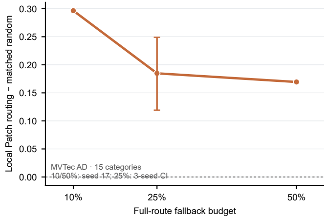
Recall difference at 5% FPR
