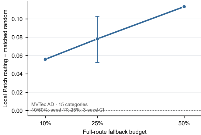
Image-level AUROC difference
