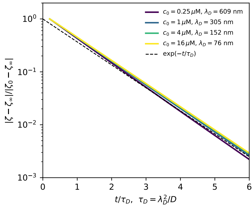
(a) one exponential, on \lambda_D^2/D
