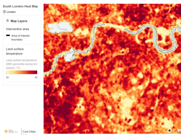
Figure 3. Land surface temperature, 95th percentile hot season (°C). Source: WRI (2026).
