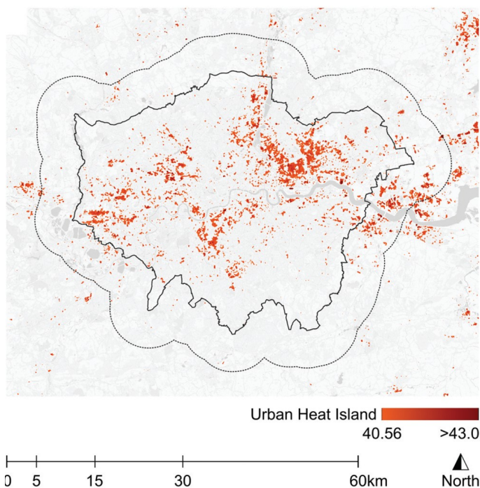
Figure 2. Urban heat island areas, Greater London, 2013 to 2023. Source: Krenz and Amann (2025), Figure 2b, CC BY 4.0.
