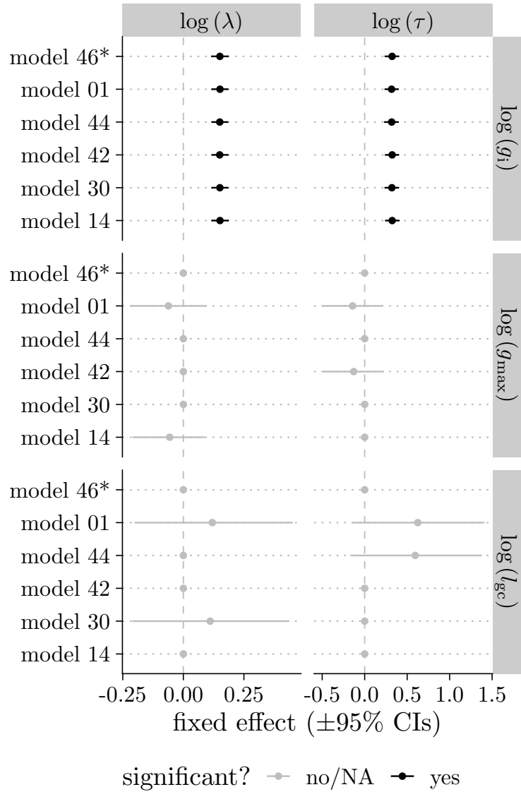
Figure S8: Individual-level (fixed-effect) estimates of guard cell length ( l_{gc} ), initial stomatal conductance ( g_i ), and anatomical maximum stomatal conductance ( g_{\max} ) on the stomatal closure time-constant ( \tau ) and lag-time ( \lambda ) are broadly consistent across all plausible models. Points and horizontal bars are posterior medians and 95% credible intervals from each of the six plausible models (rows; Table S4), ordered by \Delta\text{LOOIC} ; the selected model is marked with an asterisk (*). Black indicates estimates whose 95% credible interval excludes zero; grey indicates intervals that overlap zero.
