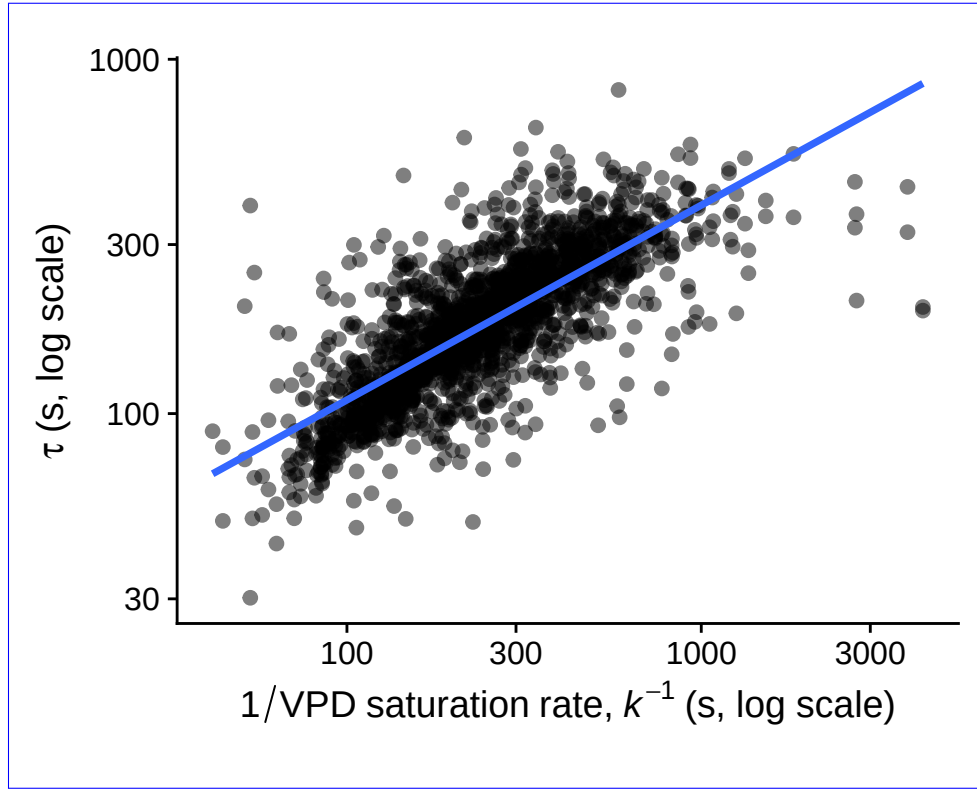
Figure S2: The stomatal closure time constant \tau (log scale) is strongly correlated with the inverse of the VPD saturation rate k^{-1} ( r = 0.77 on log-log scale). This is consistent with k being driven largely by the same g_{sw} -decline signal that determines \tau , rather than an independent property of the VPD stimulus (see Notes S1). Each point is one humidity response curve from the untreated (amphi) leaves. The blue line is ordinary least-squares regression fit.
