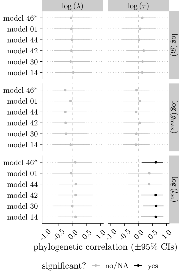
Fig. R9: Phylogenetic correlations between guard cell length ( l_{gc} ), initial stomatal conductance ( g_i ), and anatomical maximum stomatal conductance ( g_{\max} ) and the stomatal closure time constant ( \tau ) and lag time ( \lambda ), across all six plausible models identified by LOOIC (Table S4 in the manuscript). Points and horizontal bars are posterior medians and 95% credible intervals of the phylogenetic correlation; the selected model is marked with an asterisk (*). Black indicates estimates whose 95% credible interval excludes zero; grey indicates intervals that overlap zero.
