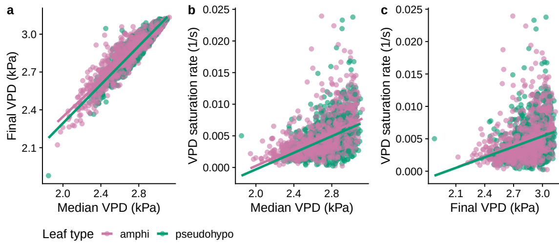
Figure S6: Pairwise relationships among curve-level VPD covariates. a. Median vs. final VPD during the fitted interval; b. median VPD vs. VPD saturation rate k ; c. final VPD vs. VPD saturation rate k . Each point is one humidity response curve, colored by leaf type; lines are ordinary least-squares fits within leaf type. VPD saturation rate is the rate constant of a saturating exponential fit to the VPD trajectory during the fitted interval (see Notes S1).
