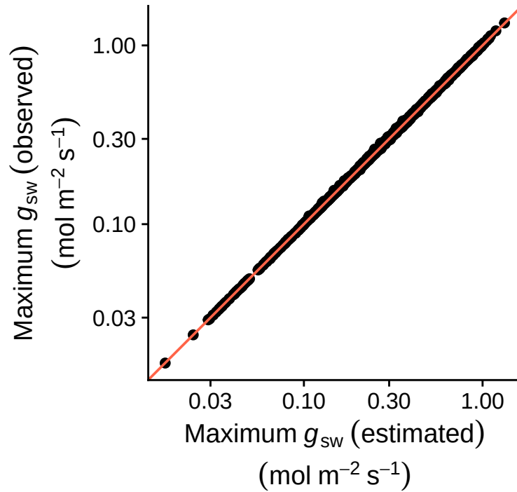
Figure S10: The estimated (x-axis) and observed (y-axis) maximum stomatal conductances ( g_{sw} ) are nearly identical. Each point is the empirical maximum g_{sw} plotted against the estimated g_{sw} for every humidity response curve. The orange line is the 1:1 line for reference. Both axes are on a log-scale.
