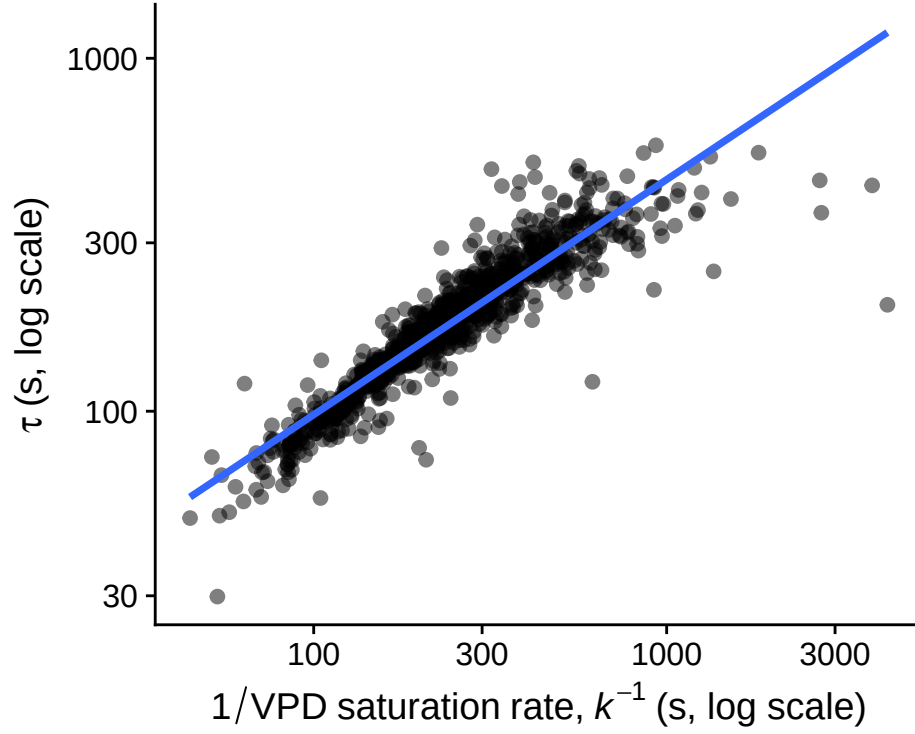
Figure S7: The stomatal closure time-constant \tau (log scale) is strongly correlated with the inverse of the VPD saturation rate k^{-1} ( r = \text{rformatC}(\text{cor\_tau\_rate}, \text{format} = 'f', \text{digits} = 2) on log-log scale). This is consistent with k being driven largely by the same g_{sw} -decline signal that determines \tau , rather than an independent property of the VPD stimulus (see Notes S1). Each point is one humidity response curve from the untreated (amphi) leaves. The blue line is ordinary least-squares regression fit.
