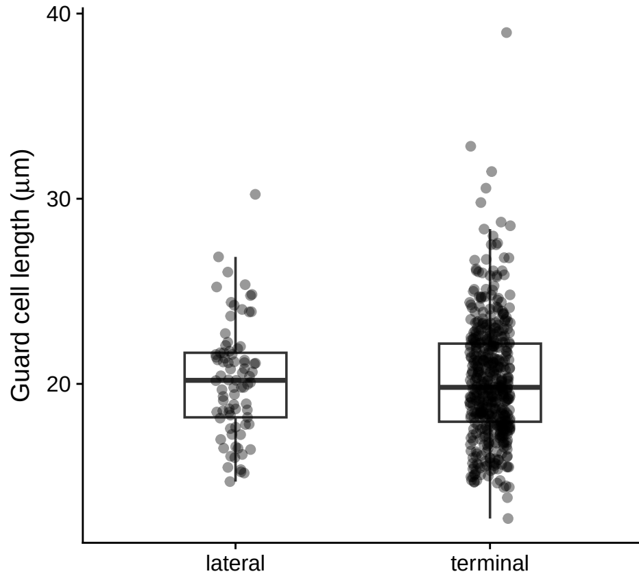
Figure S5: Lateral and terminal leaflets show at most a small, marginally detectable difference in l_{gc} . l_{gc} for lateral vs. terminal leaflets, among individuals with an amphistomatous curve; the fitted difference between leaflet types (accounting for accession and growth light treatment) is used to correct l_{gc} and g_{max} when the anatomy leaflet did not match the LI-6800 leaflet (see Materials and Methods).
