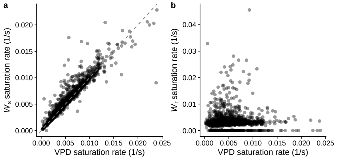
Figure S8: The VPD saturation rate is driven by the sample airstream, not the reference airstream. a. VPD saturation rate vs. the saturation rate of W_s (sample cell water vapor concentration); the dashed line is the 1:1 line. b. VPD saturation rate vs. the saturation rate of W_r (reference cell water vapor concentration, upstream of the leaf). Each point is one humidity response curve; rate constants come from the same saturating-exponential model used for VPD.
