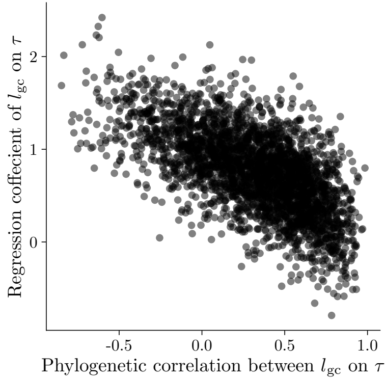
Figure S13: Posterior estimates of phylogenetic correlations ( x -axis) and fixed effects ( y -axis) of guard cell length ( l_{gc} ) on the time-constant ( \tau ) are colinear. Each point is the estimate from one draw of the posterior distribution for both parameters from the model with the lowest LOOIC. The negative relationship indicates that there is tradeoff in fitting the relationship between variables as a higher level phylogenetic effect versus a lower level, individual effect. This results in more uncertainty and larger confidence intervals in each individual parameter.
