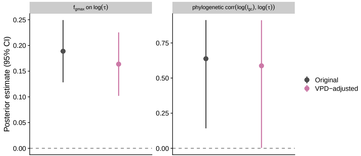
Figure S9: The f_{gmax} effect on \tau and the phylogenetic correlation between l_{gc} and \tau are robust to accounting for final VPD. Posterior means and 95% credible intervals for the fixed effect of f_{gmax} on \log \tau (left) and the phylogenetic correlation between \log l_{gc} and \log \tau (right), comparing the original model (grey) to a model refit with final VPD added as a covariate of \tau and \lambda (pink; see Notes S1).
