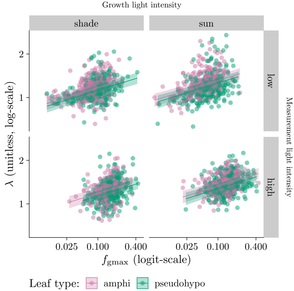
Figure S14: Individual-level variation in stomatal apertures influences stomatal closures kinetics.
