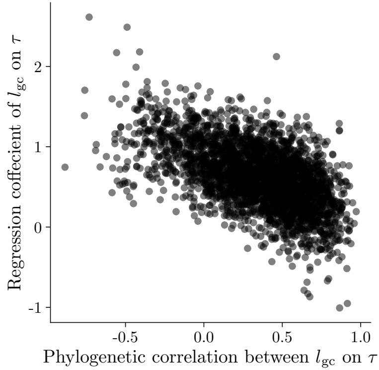
Figure S10: Posterior estimates of phylogenetic correlations ( x -axis) and fixed effects ( y -axis) of guard cell length ( l_{gc} ) on the time-constant ( \tau ) are colinear. Each point is the estimate from one draw of the posterior distribution for both parameters from the model with the lowest LOOIC. The negative relationship indicates that there is tradeoff in fitting the relationship between variables as a higher level phylogenetic effect versus a lower level, individual effect. This results in more uncertainty and larger confidence intervals in each individual parameter.
