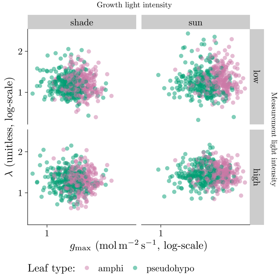
Figure S13: Individual-level variation in anatomical maximum stomatal conductance ( g_{\max} ) influences stomatal closures kinetics. As g_{\max} ( x -axis) increases, the stomatal closure lag-time ( \lambda , y -axis) decreases. The overall pattern was consistent across growth light intensity treatments (left and right facets), measurement light intensity treatments (top and bottom facets), and leaf types (point colors). Lines are estimated using linear regression along with 95% confidence ribbons. The growth and measurement light intensity treatments are described in the Materials and Methods section.
