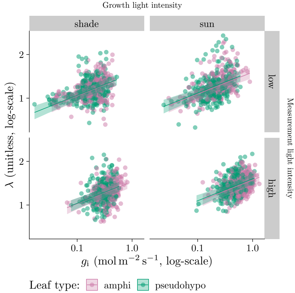
Figure S12: Individual-level variation in initial stomatal conductance ( g_i ) influences stomatal closures kinetics. As g_i ( x -axis) increases, the stomatal closure lag-time ( \lambda , y -axis) increases. The overall pattern was consistent across growth light intensity treatments (left and right facets), measurement light intensity treatments (top and bottom facets), and leaf types (point colors). Lines are estimated using linear regression along with 95% confidence ribbons. The growth and measurement light intensity treatments are described in the Materials and Methods section.
