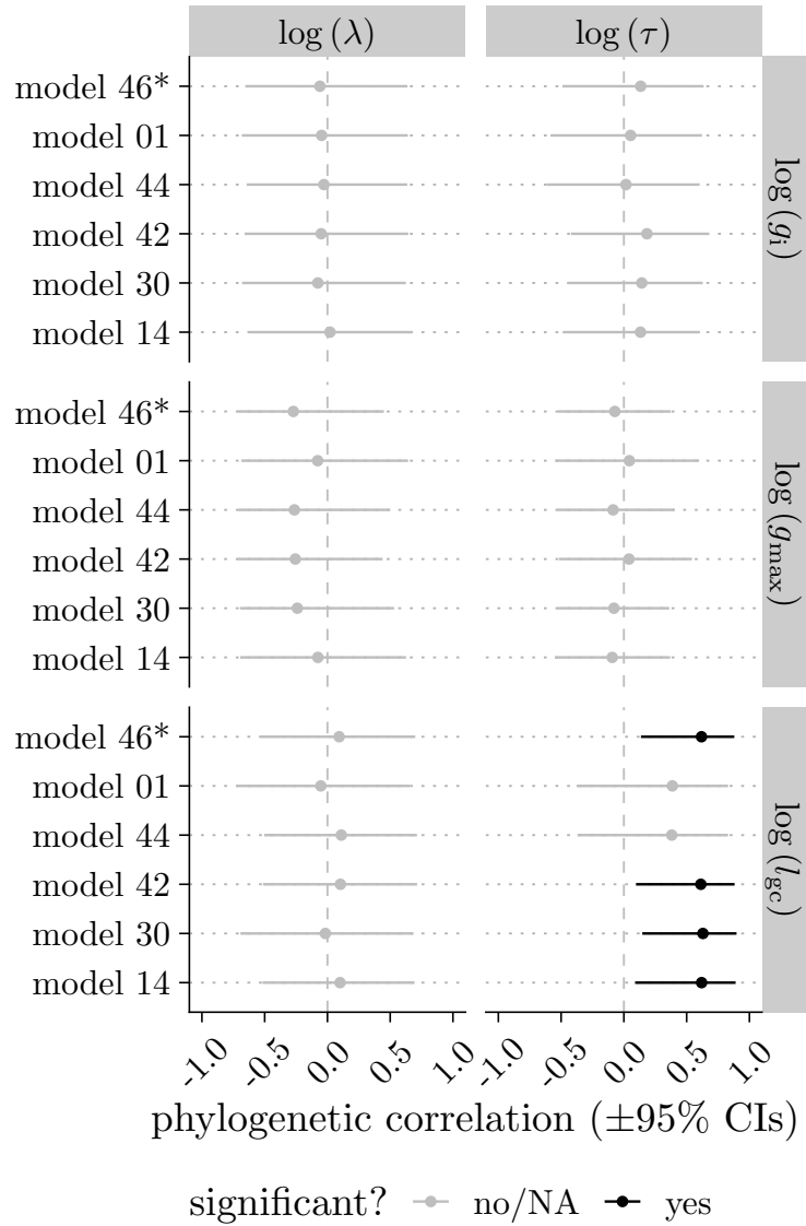
Figure S9: Phylogenetic correlations between guard cell length ( l_{gc} ), initial stomatal conductance ( g_i ), and anatomical maximum stomatal conductance ( g_{\max} ) and the stomatal closure time-constant ( \tau ) and lag-time ( \lambda ) are broadly consistent across all plausible models. Points and horizontal bars are posterior medians and 95% credible intervals of the phylogenetic correlation from each of the six plausible models (rows; Table S4), ordered by \Delta\text{LOOIC} ; the selected model is marked with an asterisk (*). Black indicates estimates whose 95% credible interval excludes zero; grey indicates intervals that overlap zero.
