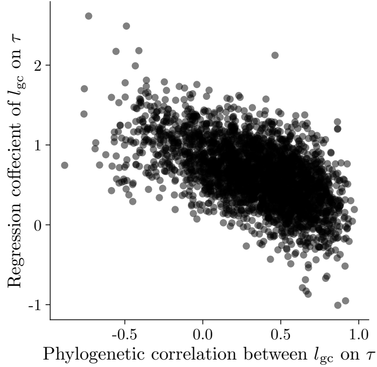
Figure S8: Posterior estimates of phylogenetic correlations ( x -axis) and fixed effects ( y -axis) of guard cell length ( l_{gc} ) on the time-constant ( \tau ) are colinear. Each point is the estimate from one draw of the posterior distribution for both parameters from the model with the lowest LOOIC. The negative relationship indicates that there is tradeoff in fitting the relationship between variables as a higher level phylogenetic effect versus a lower level, individual effect. This results in more uncertainty and larger confidence intervals in each individual parameter.
