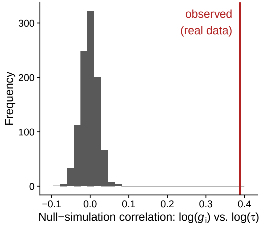
Figure S12: The curve-fitting procedure alone does not induce a g_i - \tau association. Null distribution of the correlation between estimated g_i and estimated \tau across 1,000 simulated datasets in which the true g_i and g_f are fixed at their real median values for every curve (so g_i has no true relationship with \tau by construction), compared to the observed correlation in the real data (red line).
