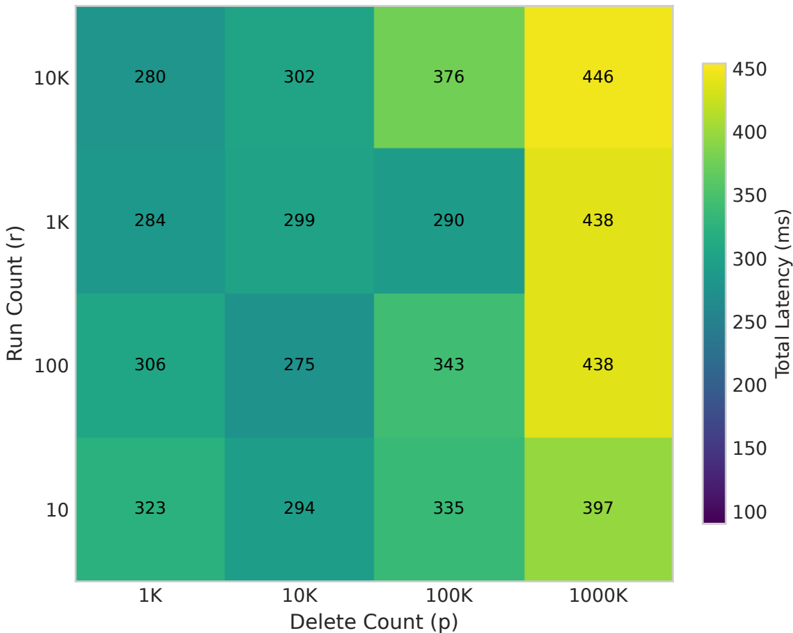
Total Latency: GCP (Deletion Vectors)
