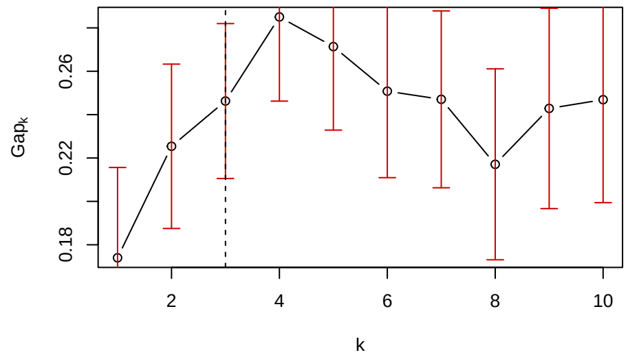
Gap statistic
