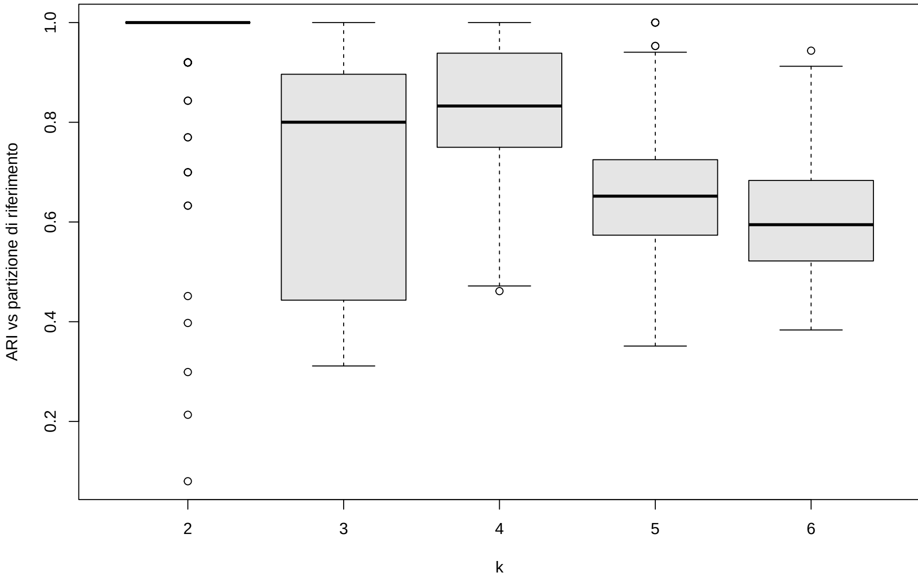
Stabilita' bootstrap (B = 200)
