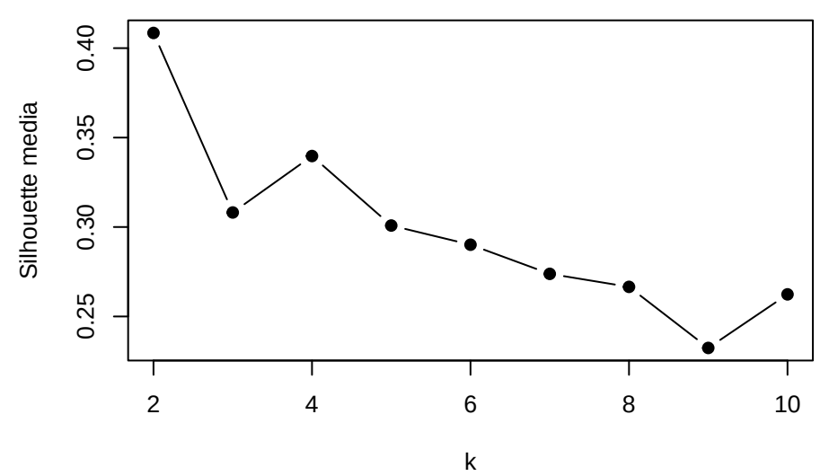
Silhouette media
