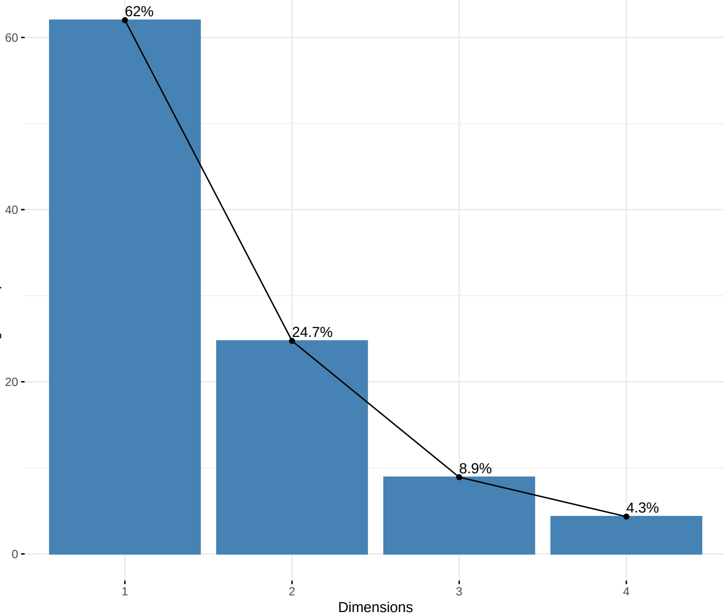
Scree plot
