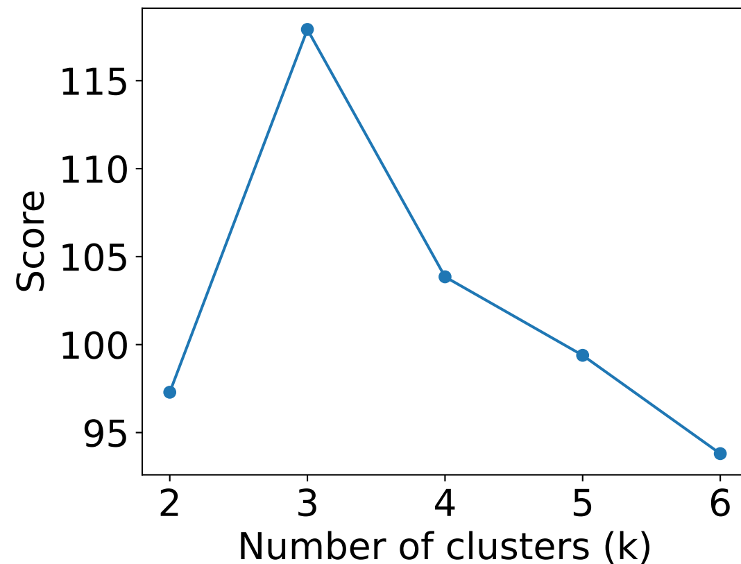
Calinski-Harabasz index
