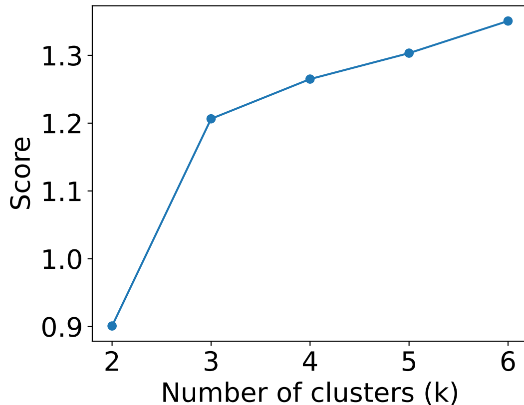
Davies-Bouldin index
