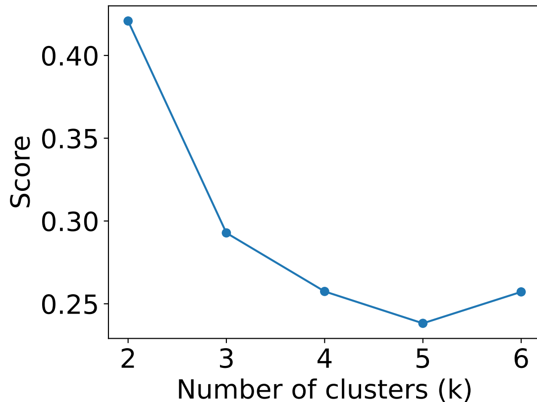
Silhouette score
